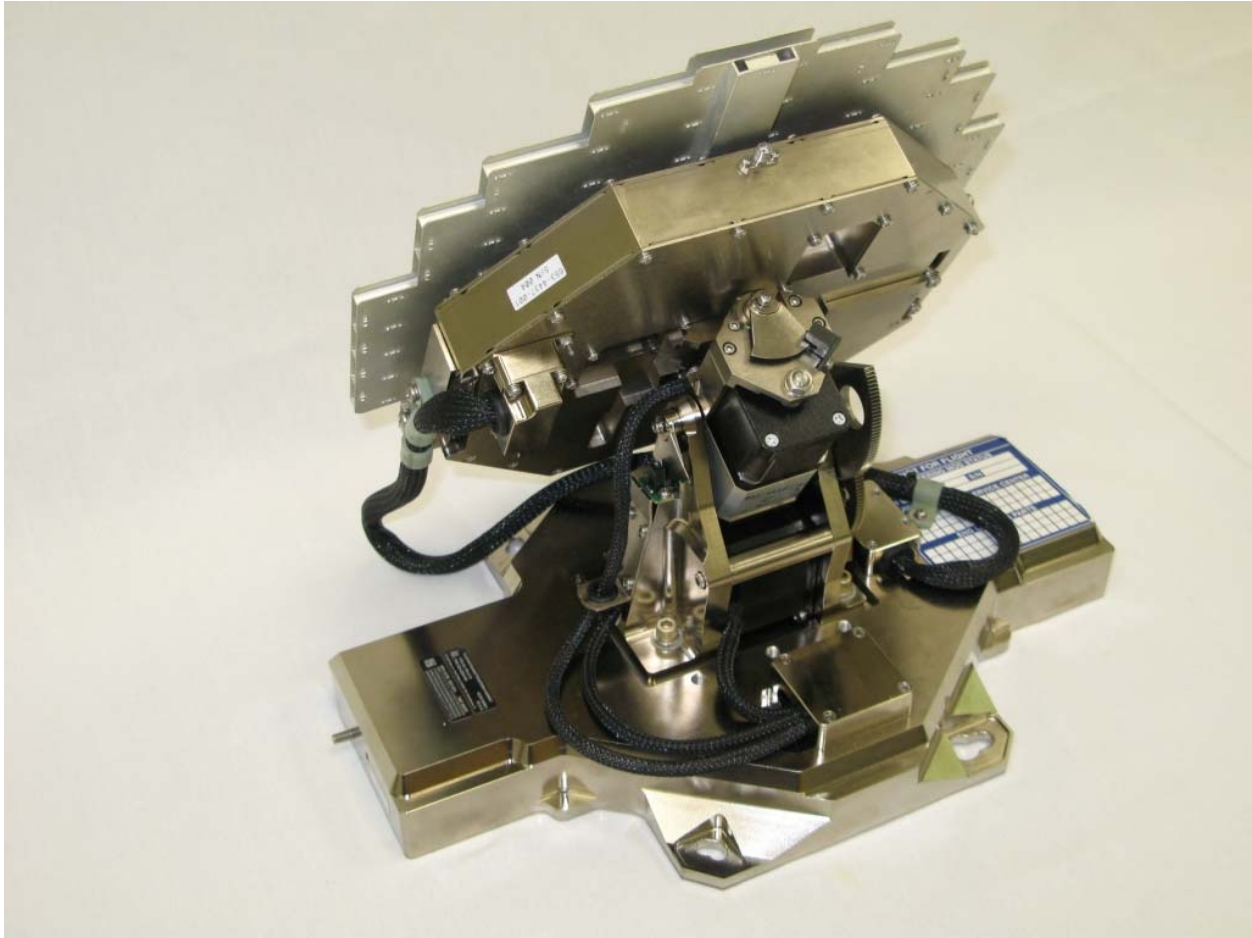
Figure C-1 – RTA-4112 External Photograph - Side
