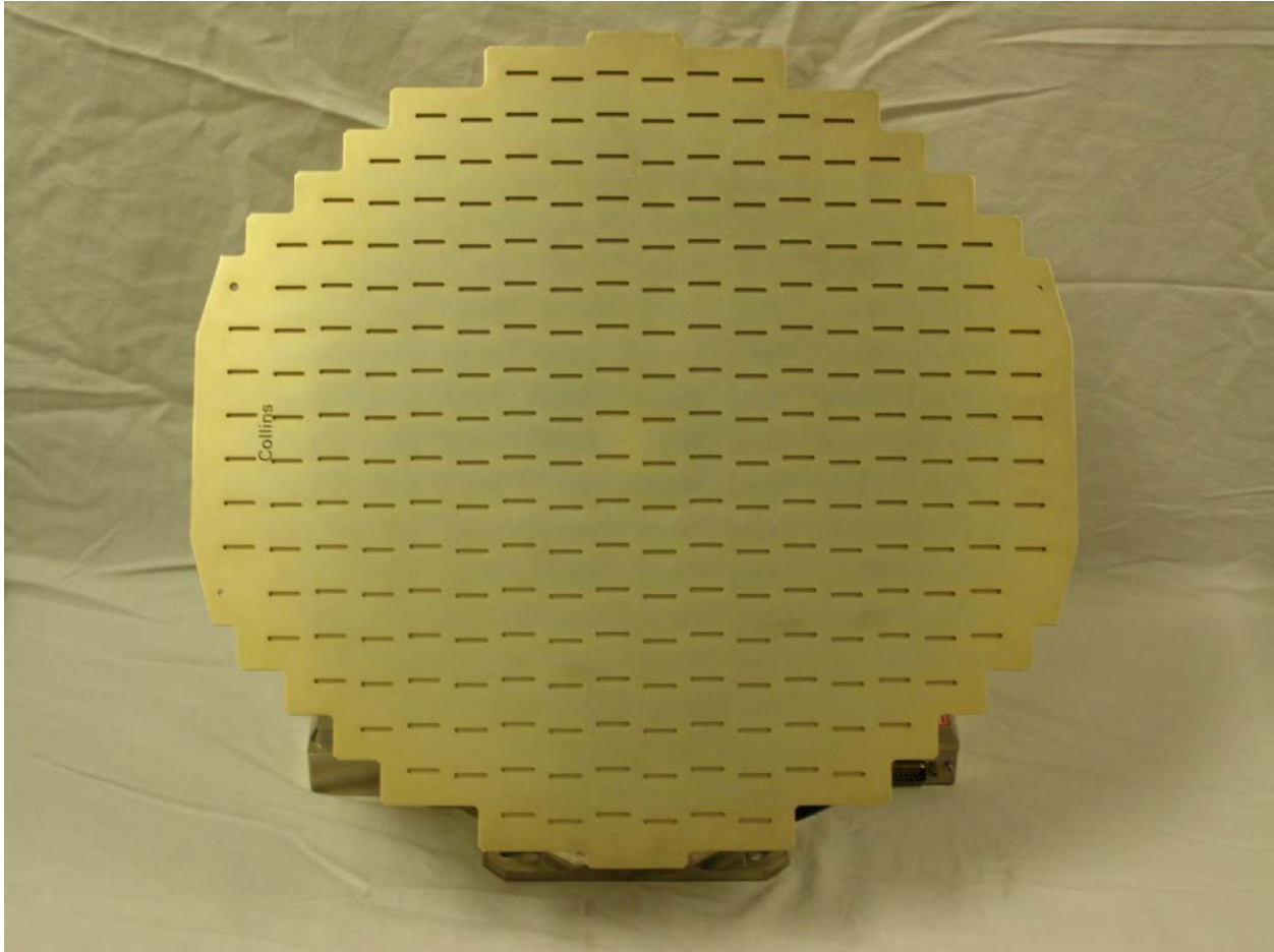
Figure C-6 – RTA-4118 External Photograph - Antenna
