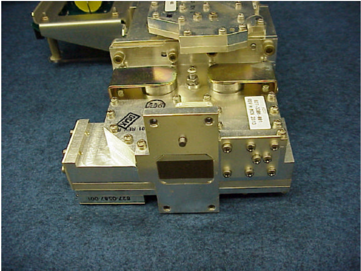
Figure 8-16. Duplexer
