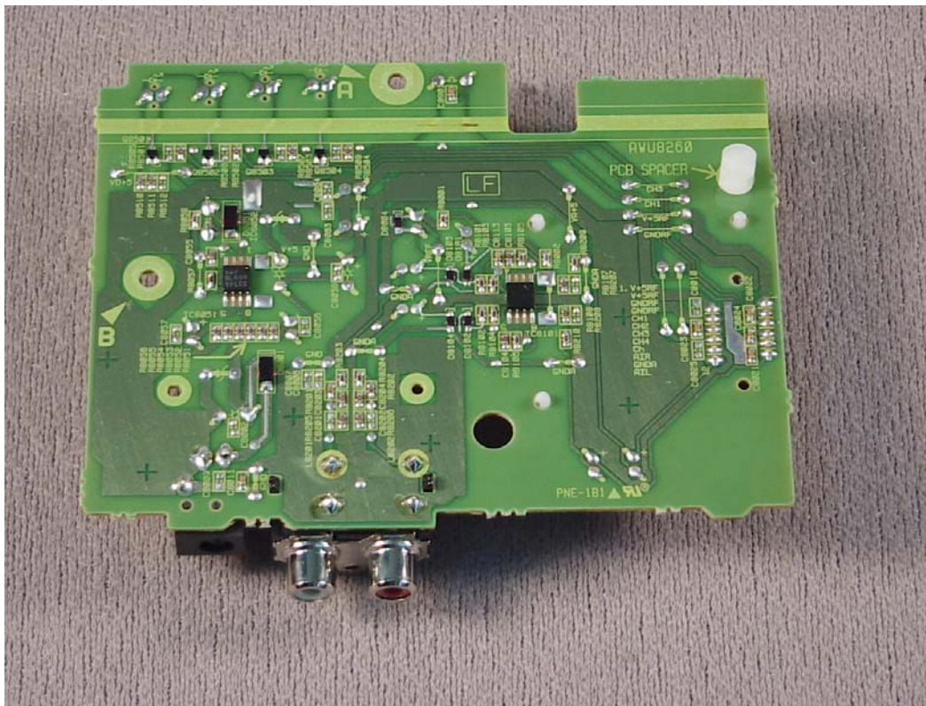
PWB Side A
