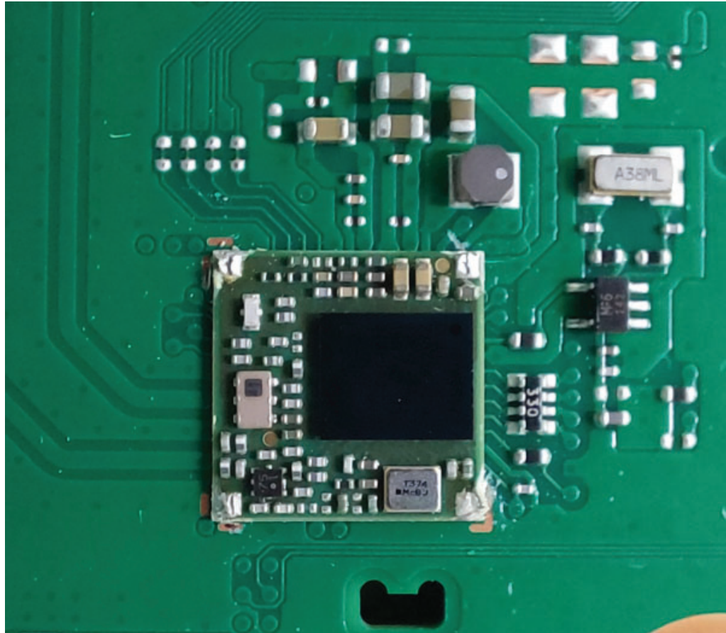
RF Module (shield case removed)
