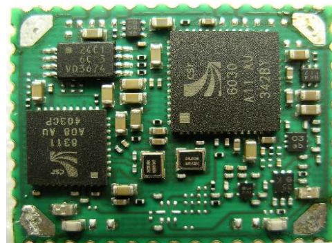
Module surface side (without shield)
