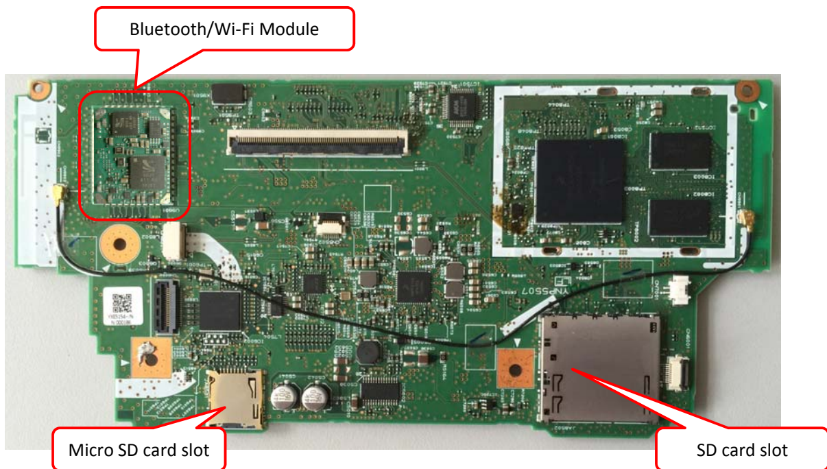
Electronic Board back side
