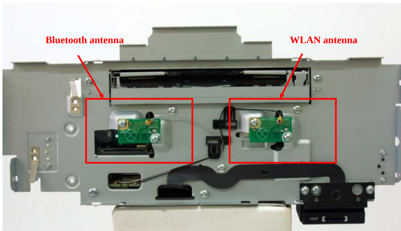
Antenna Location
