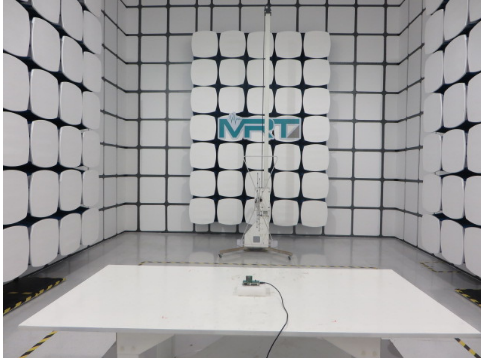
Photograph 1: Set-up for Radiated Emission, 30MHz-1000MHz
