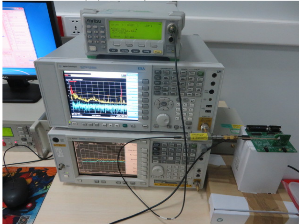
Photograph 3: Set-up for conducted RF Test
