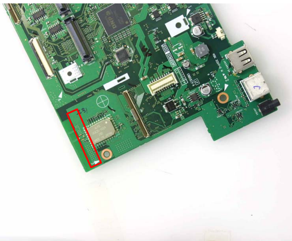
Antenna Position
