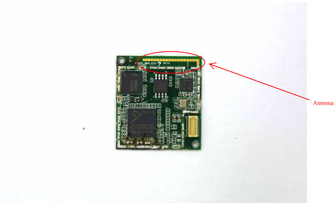
Bluetooth Board side A without shield
