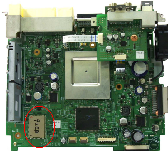
Bluetooth Board Position
