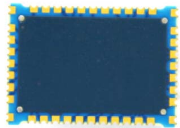
Back View of BT module
