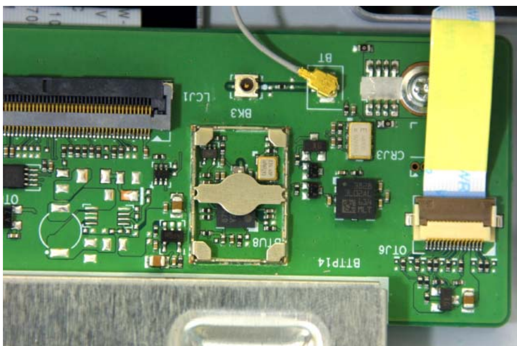
BT module Close up without Shield
