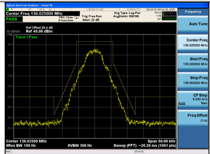
Emission Mask D@173.975MHz-2W-4FSK
