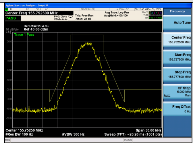
Emission Mask D@136.025MHz-2W-4FSK
