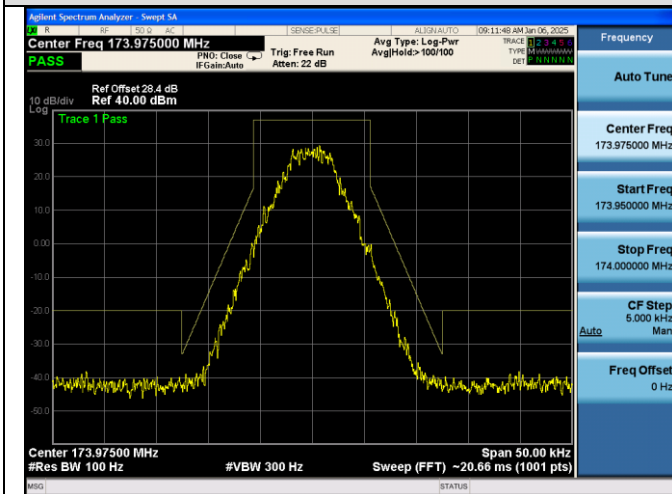
Emission Mask D@155.7525MHz-2W-4FSK
