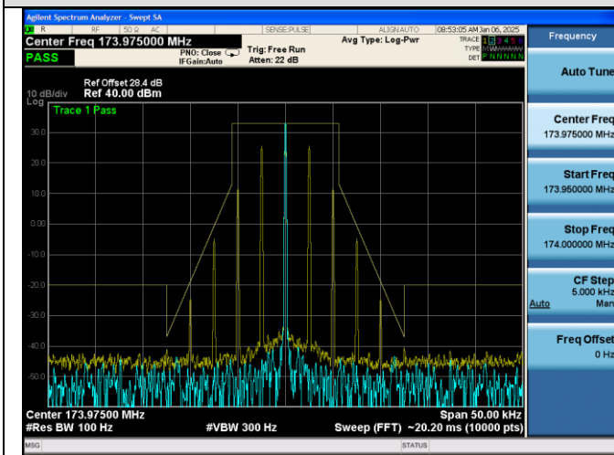
Emission Mask D@173.975MHz-5W-4FSK
