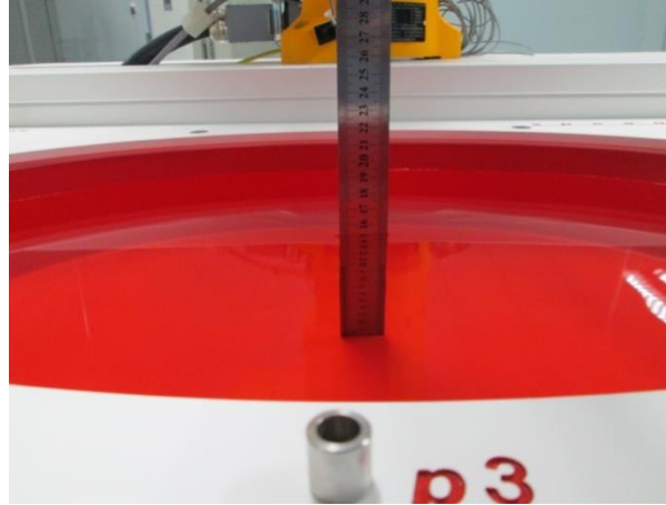
150MHz flat phantom
