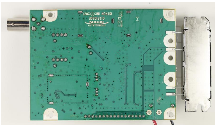
RF Board Bottom View
