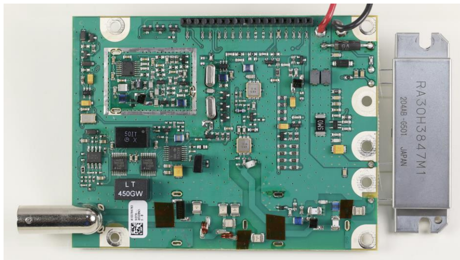
RF Board Top View w/o Shields
