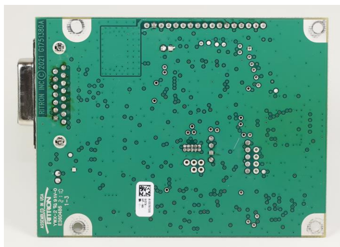
Control/Loader Board Bottom View
