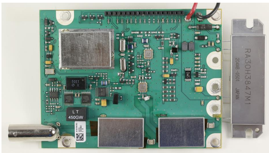
RF Board Top View w/ Shields
