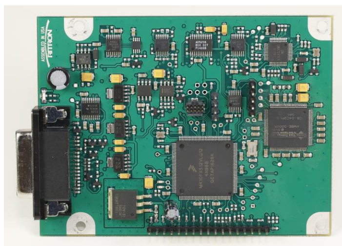
Control/Loader Board Top View
