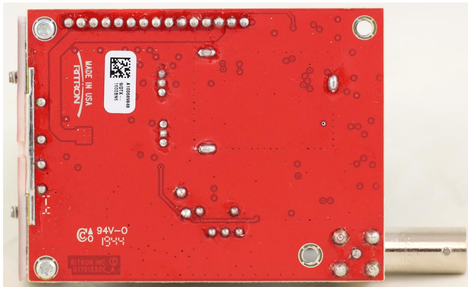
RF Board Bottom View
