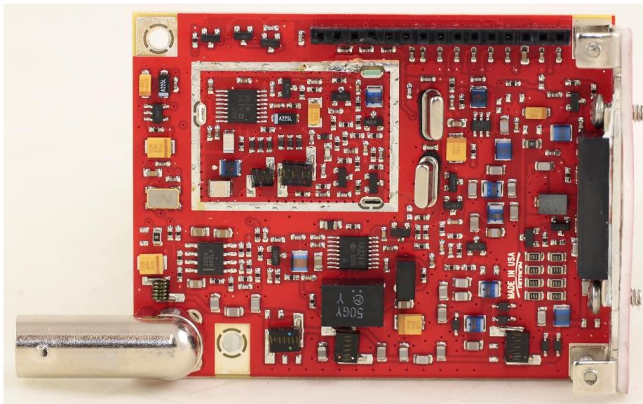
RF Board Top View w/o Shield
