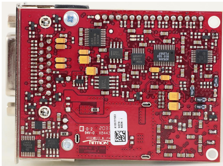
Control/Loader Board Bottom View
