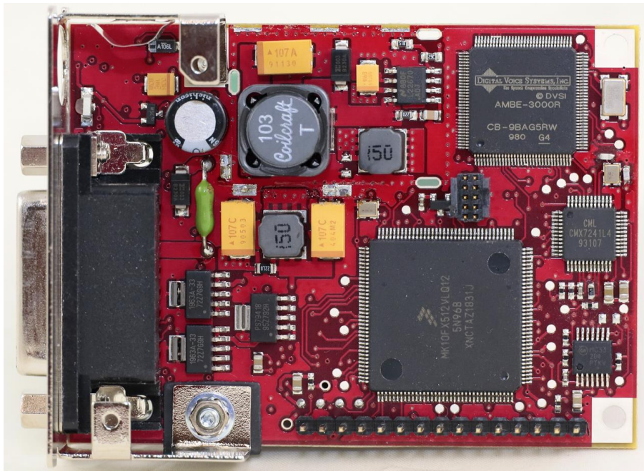
Control/Loader Board w/o Shield Top View
