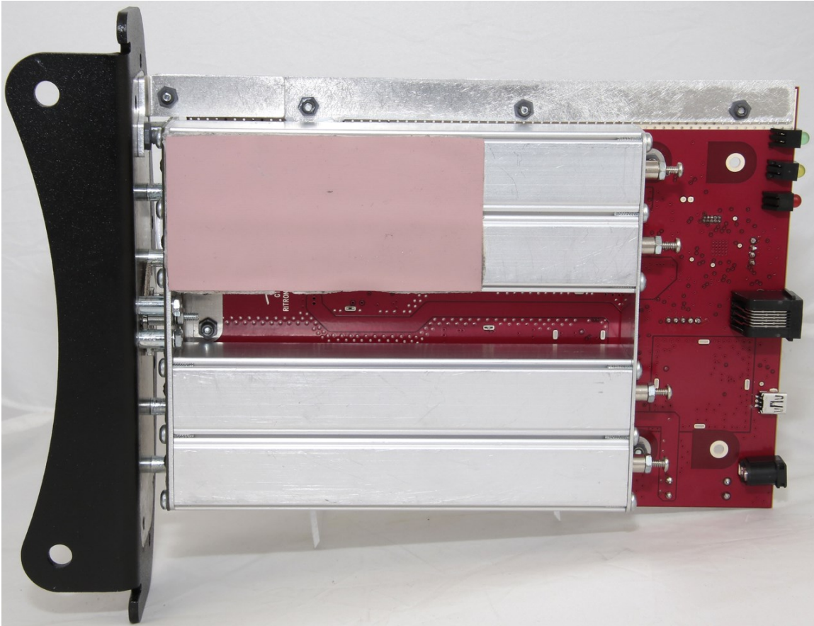
RLR-465 bottom view with duplexer and heatsink
