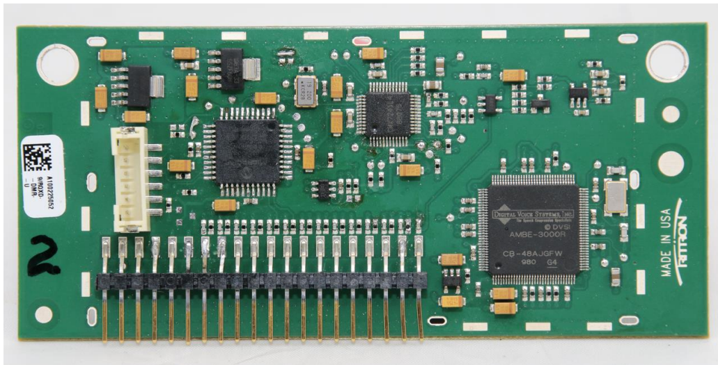
9/RQXD-DMR Top View w/o Shields
