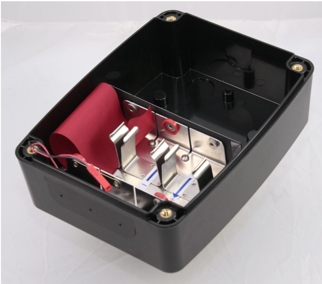
RQX-417DMR Battery Holder installed in Rear Enclosure
