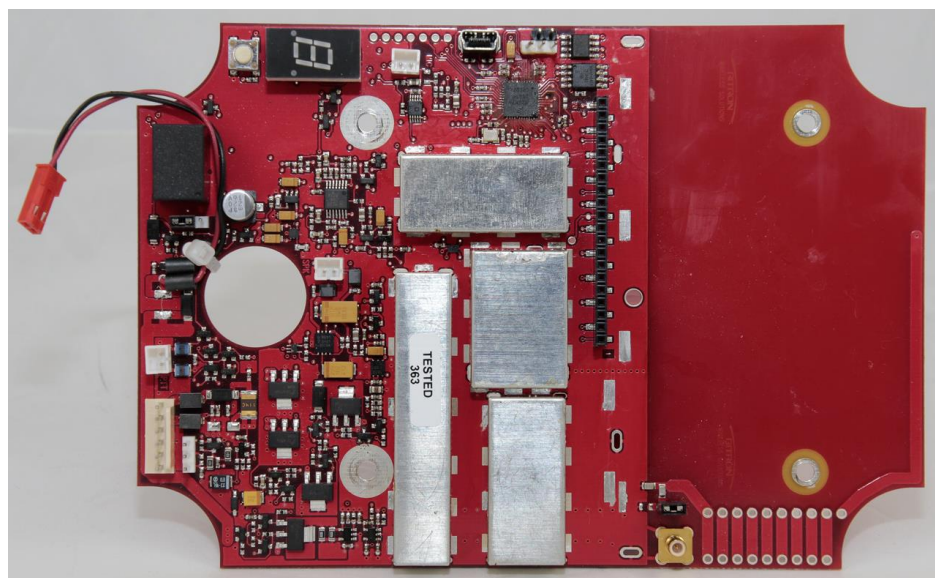
RQX-417DMR Top View w/ Shields
