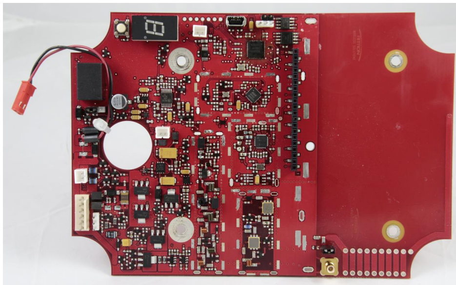
RQX-417DMR Top View w/o Shields
