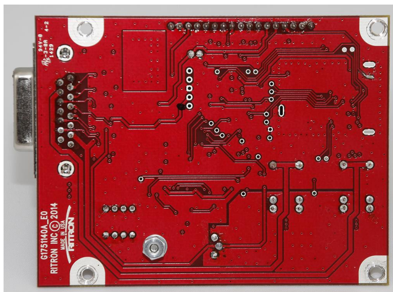
DTX-165-RR-SIG Control/Loader Board Bottom View
