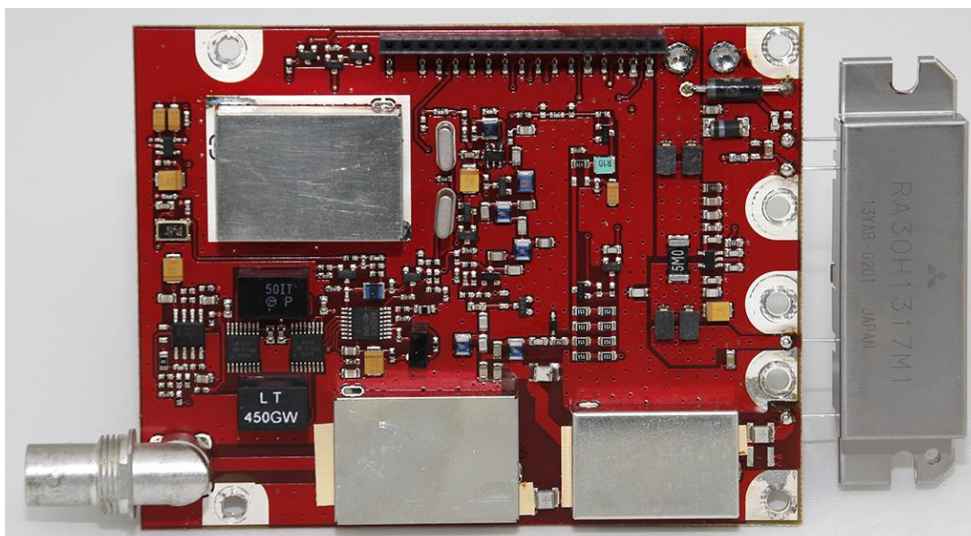
DTX-165-RR-SIG RF Board Top View w/ Shields
