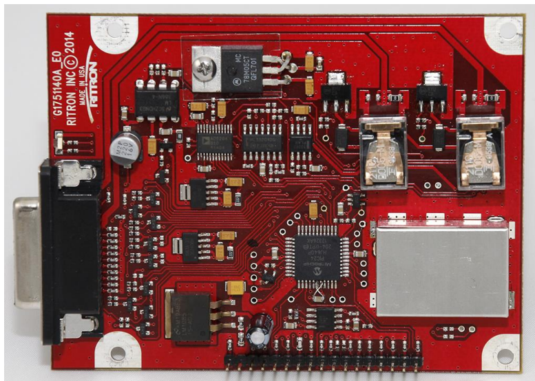
DTX-165-RR-SIG Control/Loader Board Top View w/ Shield
