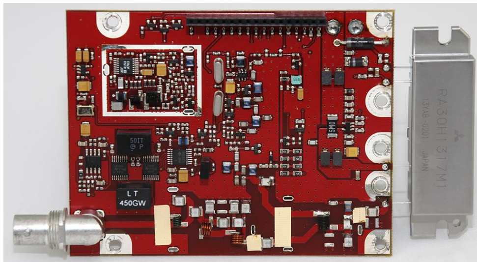
DTX-165-RR-SIG RF Board Top View w/o Shields
