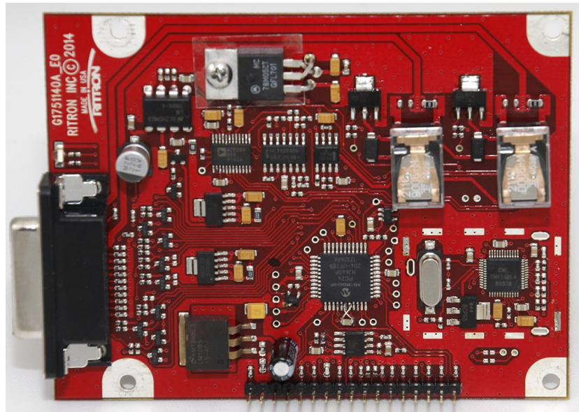
DTX-165-RR-SIG Control/Loader Board Top View w/o Shield
