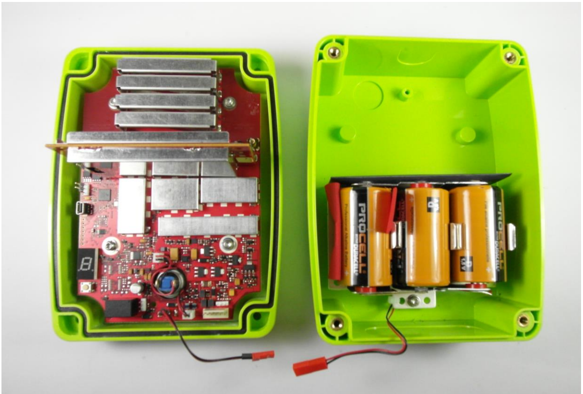
EXHIBIT: RQX-117NX with 3 D-cell batteries. Case open to show printed circuit board installation FCC ID: AIERIT41-117
