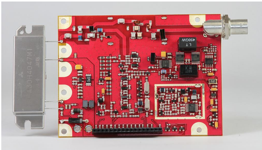
DTX-465 RF Board Top View w/o Shields
