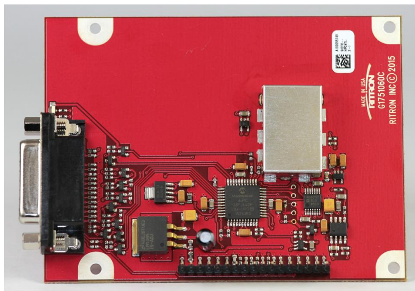
DTX-465 Control/Loader Board Top View w/ Shield
