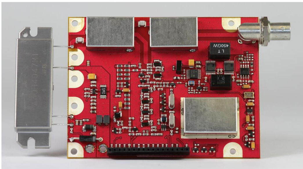
DTX-465 RF Board Top View w/ Shields
