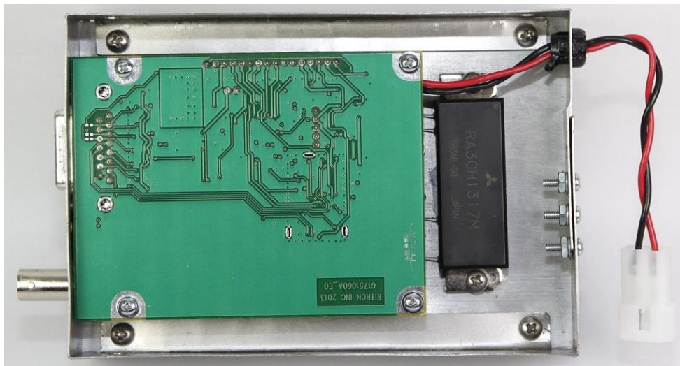
DTX-165 PCB/Heatsink Assembly w/ Enclosure Shield
