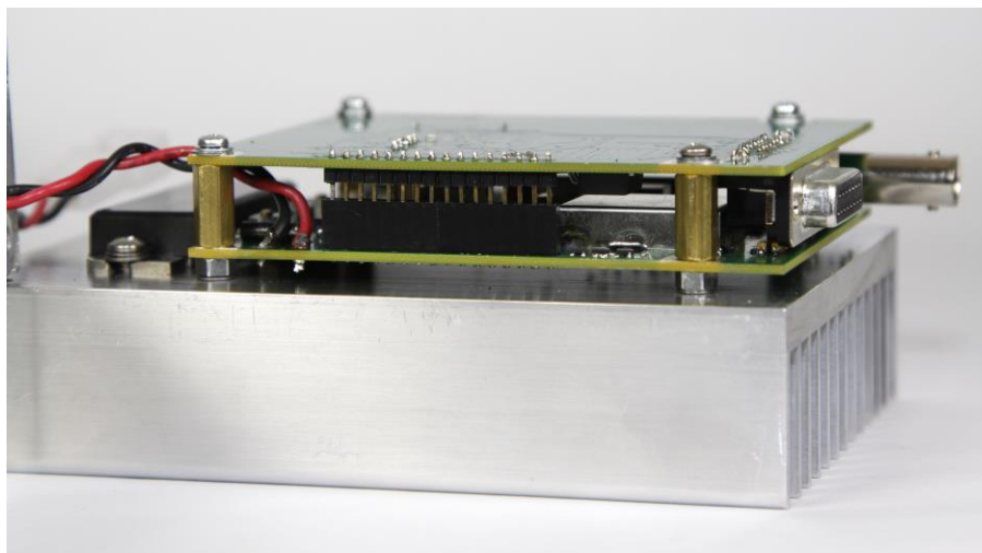
DTX-165 PCB Assembly Side View
