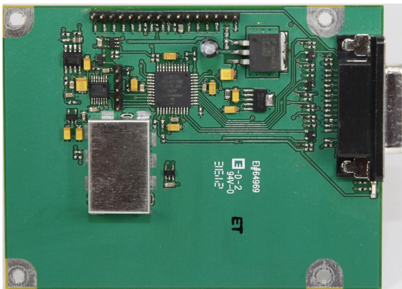
DTX-165 Control/Loader Board Top View w/ Shield
