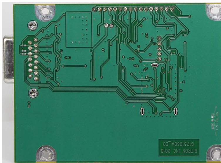
DTX-165 Control/Loader Board Bottom View
