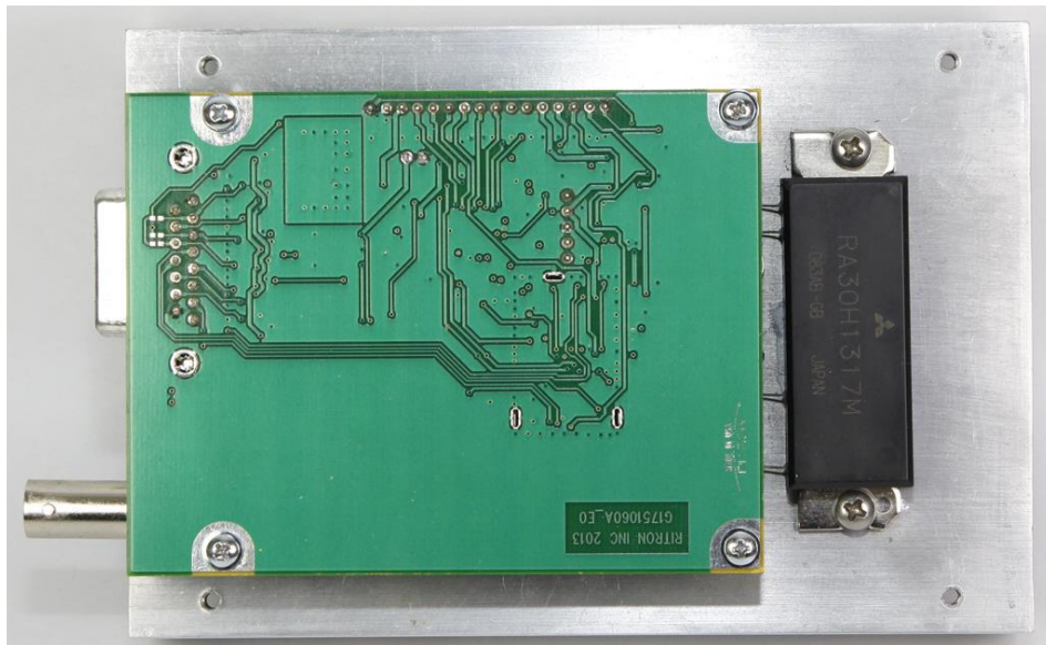
DTX-165 PCB Assembly Installed on Heatsink
