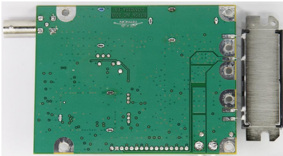
DTX-165 RF Board Bottom View
