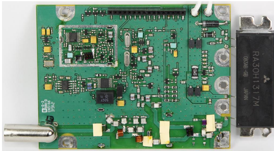
DTX-165 RF Board Top View w/o Shields
