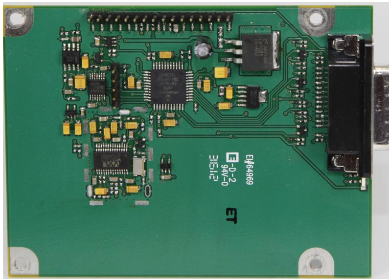
DTX-165 Control/Loader Board Top View w/o Shield
