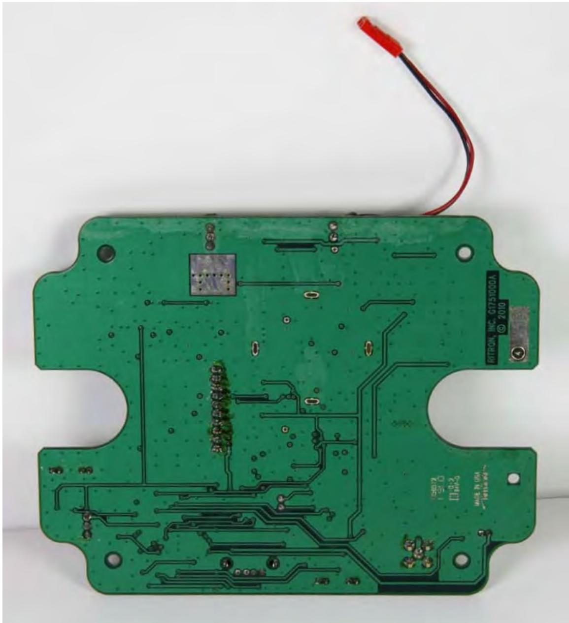
EXHIBIT: RQT-451 complete bottomside PCB assembly FCC ID: AIERIT32-451
