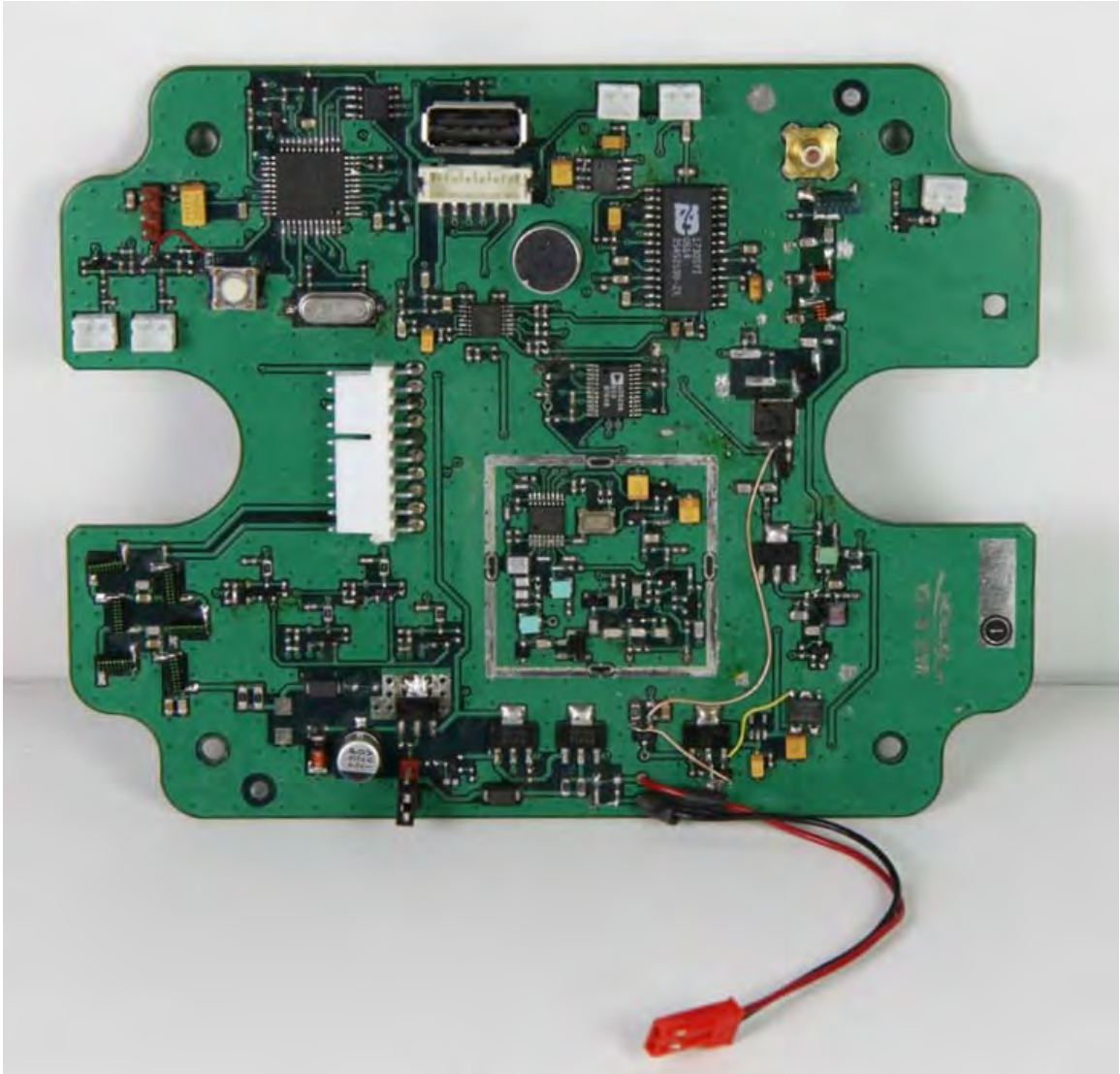
EXHIBIT: RQT-451 complete topside PCB assembly with shield removed FCC ID: AIERIT32-451
