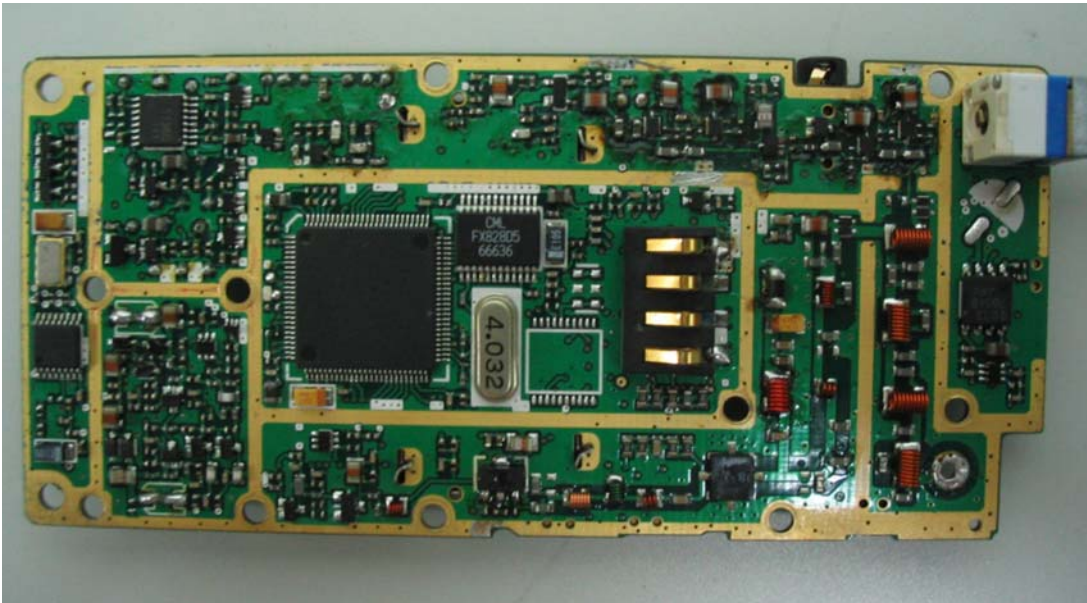
Bottomside PCB Assembly with Shields Removed
