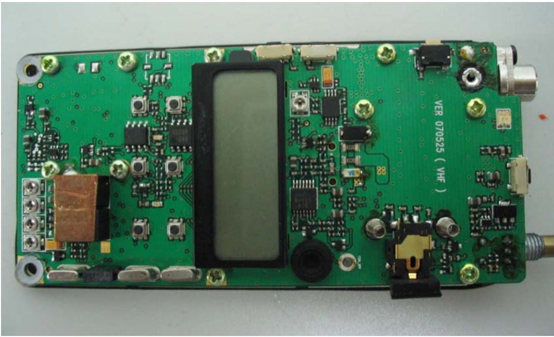
Topside PCB Assembly
