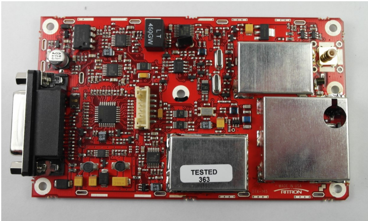
DTX-145M top side with shields
