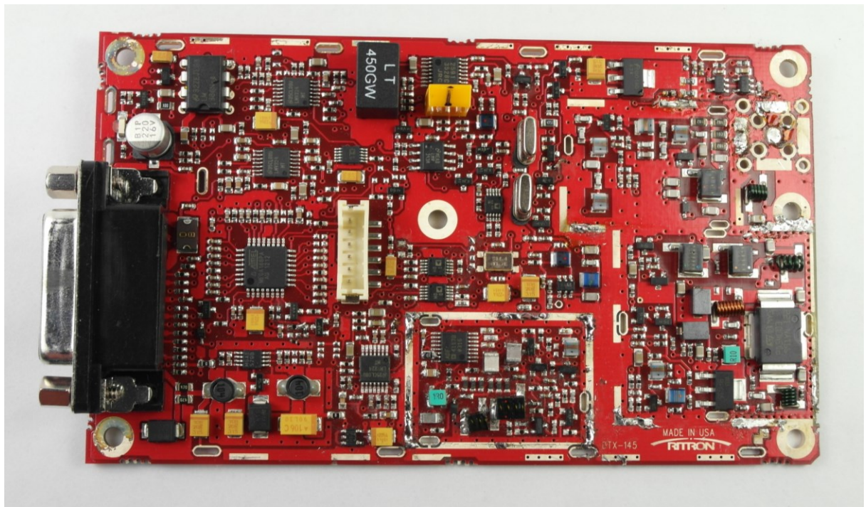
DTX-145M top side with no shields
