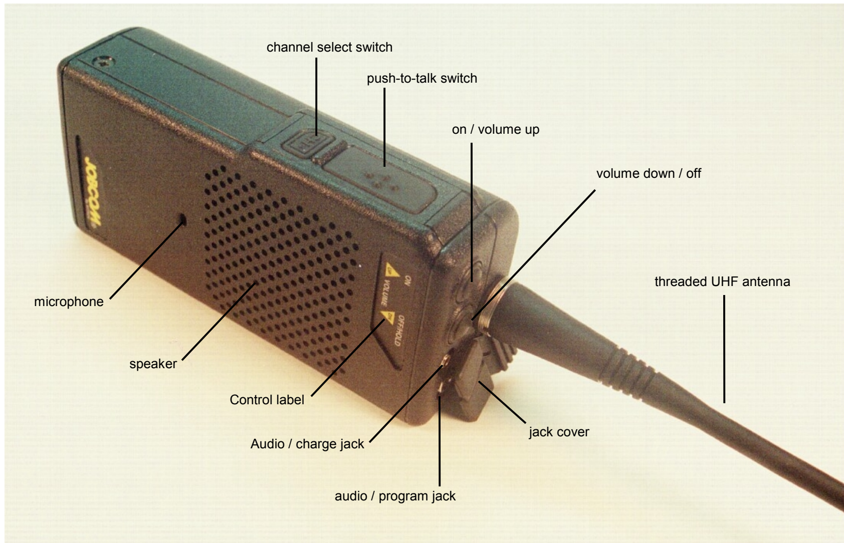
AIERIT13-442 SST-442 controls, jacks, and control label
