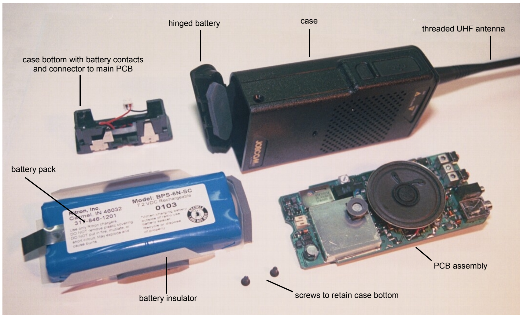
AIERIT13-442 SST-442 case assembly components
