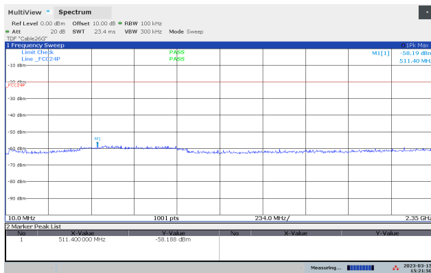
Conducted Emissions 10-2350 MHz, 2402 MHz, 1Mb
