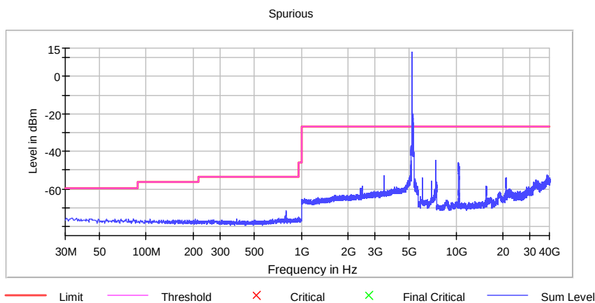
Unwanted Emissions 30M-40GHz, ch044, 802.11n HT20, MIMO, Conducted
