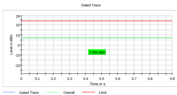
RMS Conducted Power, 5500 MHz, 802.11n, HT20, MCS0, Ant1
