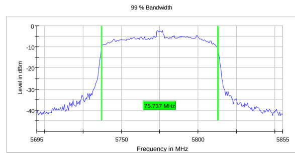
99% Occupied Bandwidth, 5775 MHz, 802.11ac, HT80
