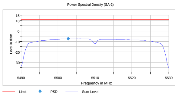
PSD, 5510 MHz, 802.11n, HT40, MCS0, Ant1 -7.5
