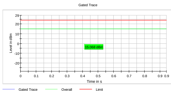
RMS Conducted Power, 5300 MHz, 802.11a, 6Mb
