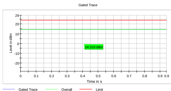
RMS Conducted Power, 5240 MHz, 802.11a, 6Mb
