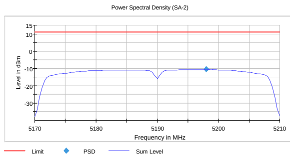
PSD, 5190 MHz, 802.11n, HT40, MCS0, Ant1 -10.5
