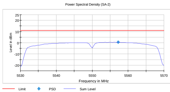
PSD, 5550 MHz, 802.11n, HT40, MCS0, Ant1 0.5
