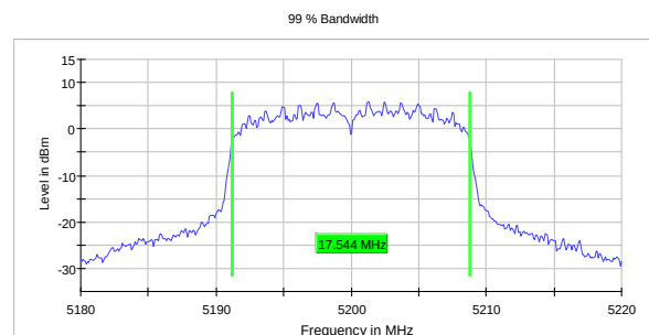
99% Occupied Bandwidth, 5200 MHz, 802.11n, HT20
