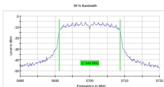
99% Occupied Bandwidth, 5700 MHz, 802.11n, HT20
