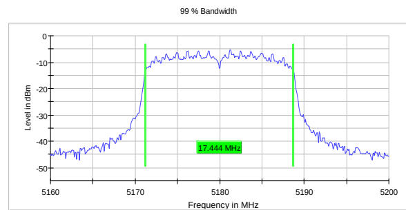
99% Occupied Bandwidth, 5180 MHz, 802.11n, HT20
