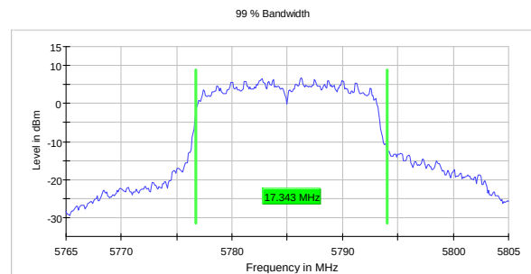
99% Occupied Bandwidth, 5785 MHz, 802.11a, 6Mb
