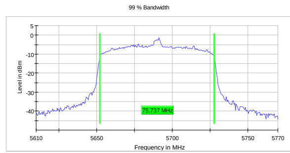
99% Occupied Bandwidth, 5690 MHz, 802.11ac, HT80
