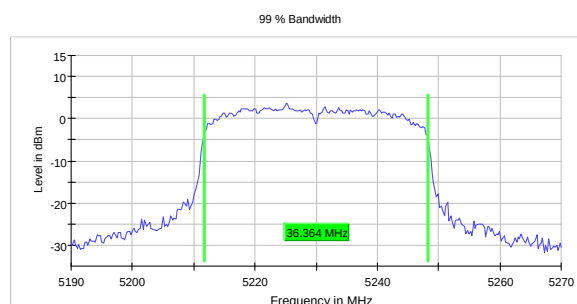
99% Occupied Bandwidth, 5230 MHz, 802.11n, HT40
