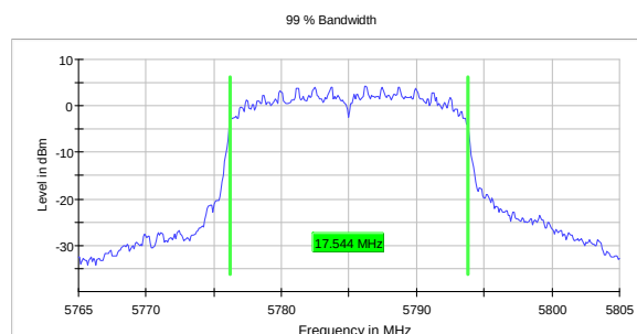
99% Occupied Bandwidth, 5785 MHz, 802.11n, HT20
