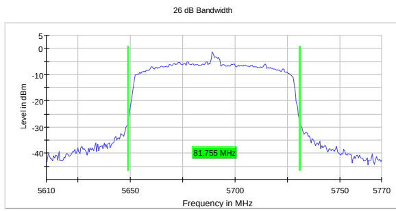
Emission Bandwidth, 5690 MHz, 802.11ac, HT80
