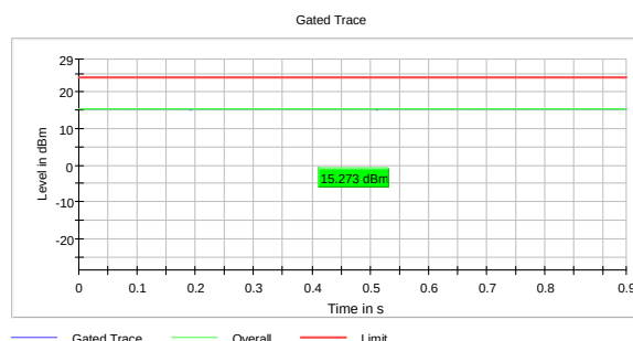
RMS Conducted Power, 5520 MHz, 802.11a, 6Mb
