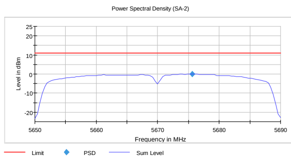
PSD, 5670 MHz, 802.11n, HT40, MCS0, Ant1 0.0
