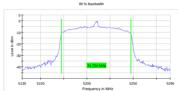
99% Occupied Bandwidth, 5210 MHz, 802.11ac, HT80
