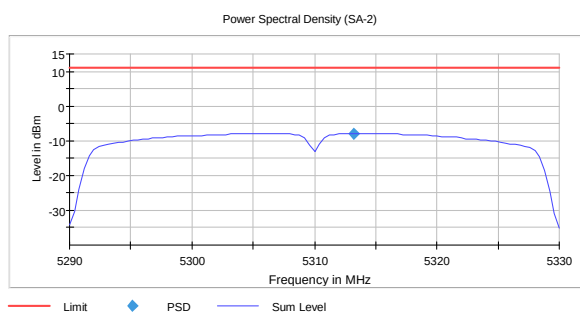
PSD, 5310 MHz, 802.11n, HT40, MCS0, Ant1 -7.9
