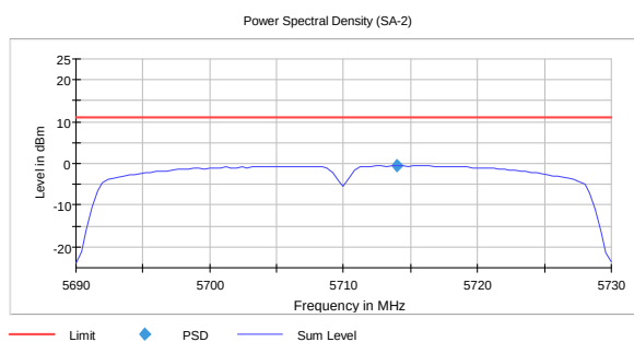
PSD, 5710 MHz, 802.11n, HT40, MCS0, Ant1 -0.5
