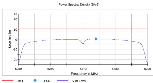
PSD, 5270 MHz, 802.11n, HT40, MCS0, Ant1 0.2
