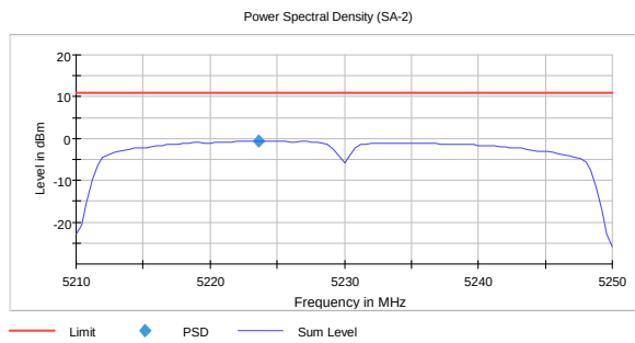
PSD, 5230 MHz, 802.11n, HT40, MCS0, Ant1 -0.6
