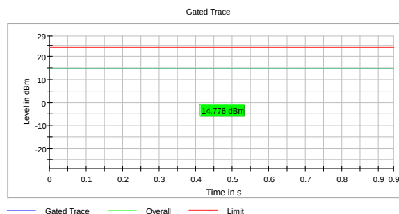
RMS Conducted Power, 5260 MHz, 802.11a, 6Mb
