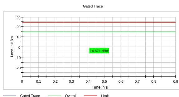
RMS Conducted Power, 5200 MHz, 802.11a, 6Mb
