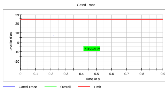
RMS Conducted Power, 5320 MHz, 802.11a, 6Mb
