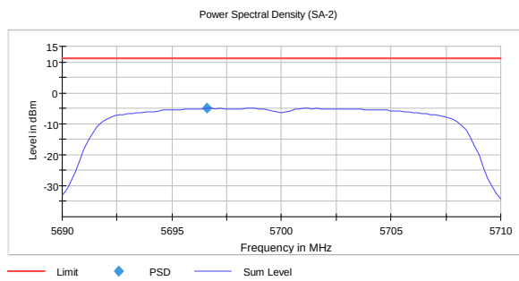
PSD, 5700 MHz, 802.11a, 6Mb -5.0
