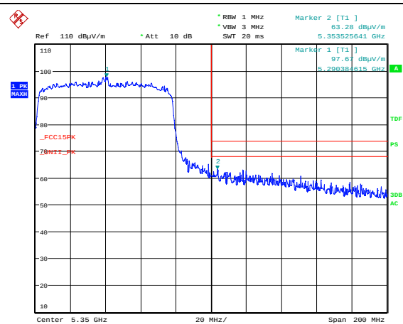
Band Edge 5350 MHz, ch058, 802.11ac HT80 MIMO, Radiated, Max, Pk
