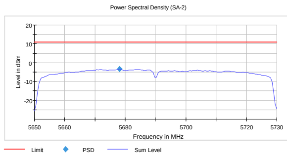
PSD, 5690 MHz, 802.11ac, HT80, Ant1, -3.5
