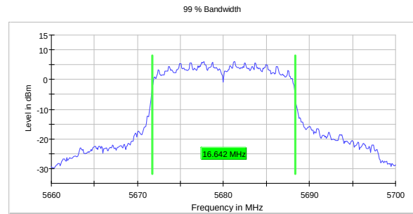
99% Occupied Bandwidth, 5680 MHz, 802.11a, 6Mb
