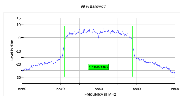
99% Occupied Bandwidth, 5580 MHz, 802.11n, HT20
