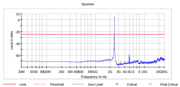
Conducted Emissions Ch06, 802.11g 6M
