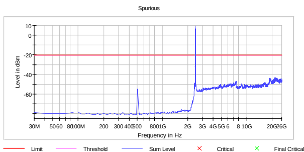
Conducted Emissions Ch10, 802.11b 11M
