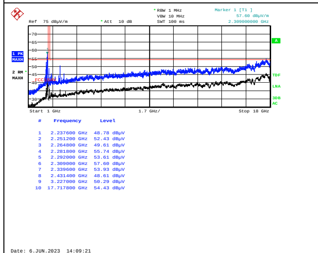
Radiated Emissions 1 - 18 GHz, Ch06, 802.11n HT40, MIMO, HP
