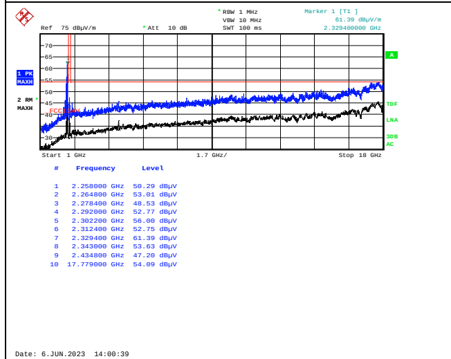
Radiated Emissions 1 - 18 GHz, Ch06, 802.11n HT40, Ant1, HP
