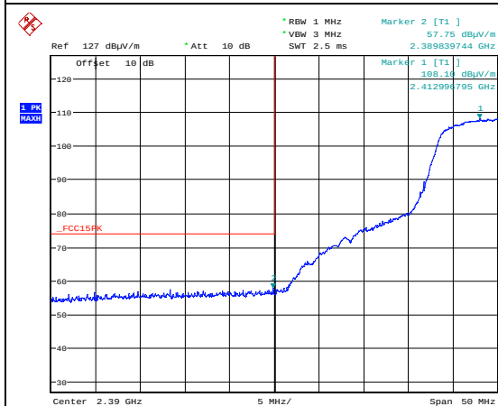
Band Edge, 2417 MHz, 802.11g 6M, Peak
