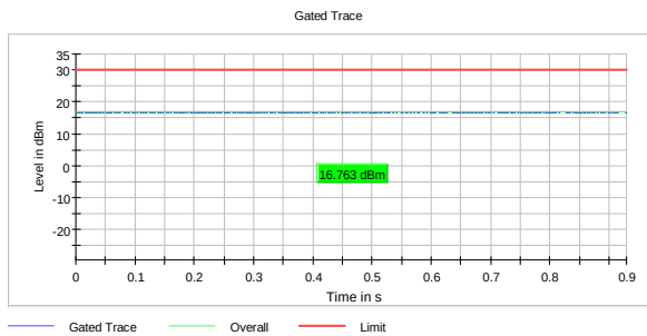
RMS Power, 2457 MHz, 802.11n MIMO MCS8
