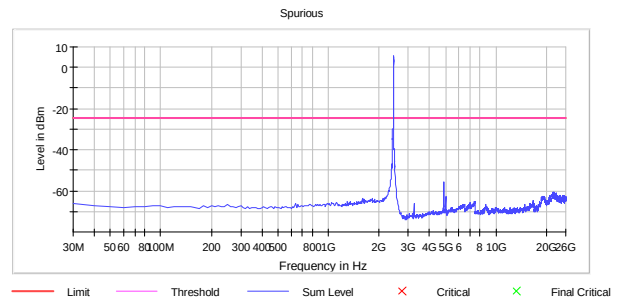
Conducted Emissions Ch06, 802.11n MCS8 MIMO
