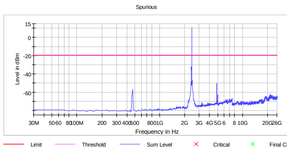
Conducted Emissions Ch06, 802.11b 11M
