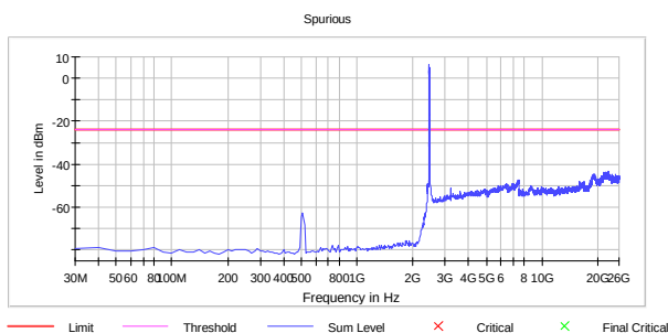
Conducted Emissions Ch10, 802.11g 6M
