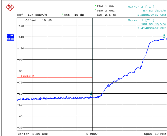
Band Edge, 2417 MHz, 802.11b 11M, Peak
