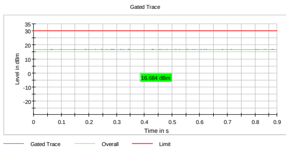
RMS Power, 2447 MHz, 802.11n HT40 MIMO MCS8
