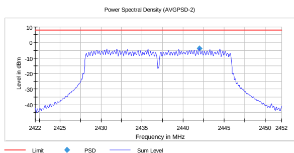
PSD, 2437 MHz, 802.11n SISO MCS7 -3.77
