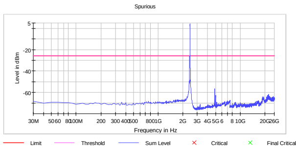
Conducted Emissions Ch06, 802.11n MCS0 SISO
