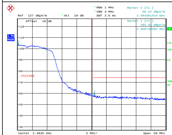
Band Edge, 2462 MHz, 802.11g 6M, Peak
