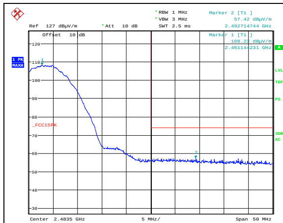
Band Edge, 2462 MHz, 802.11b 11M, Peak
