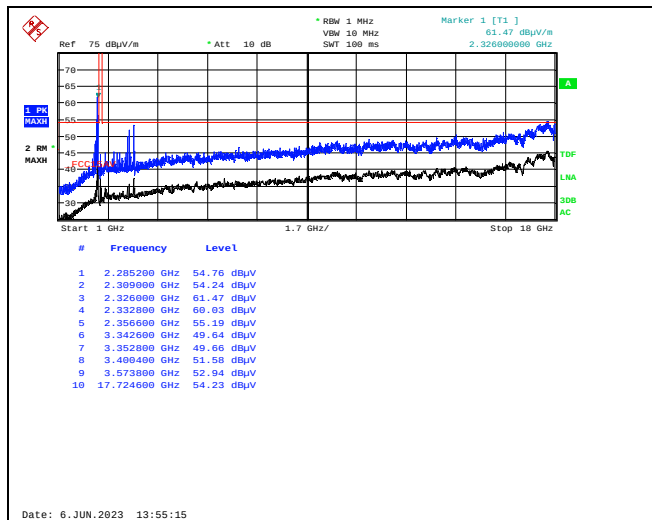
Radiated Emissions 1 - 18 GHz, Ch06, 802.11n HT40, Ant0, HP
