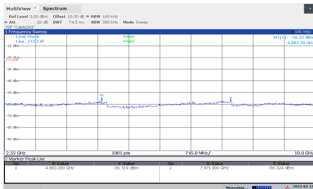
Conducted Emissions 2.55-10 GHz, 2440 MHz, 1Mb
