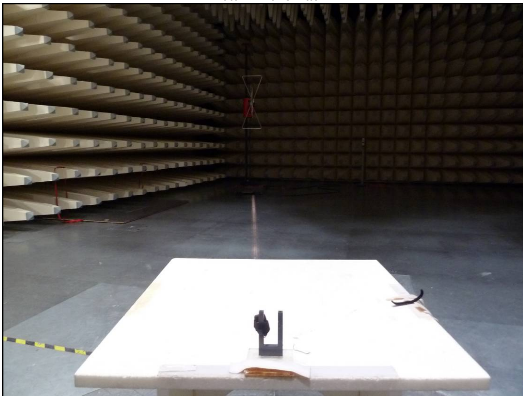
Photo 1: Transmitter
