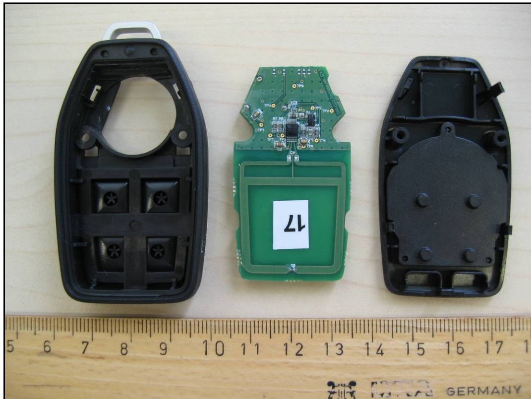
Photo 10: Transmitter
