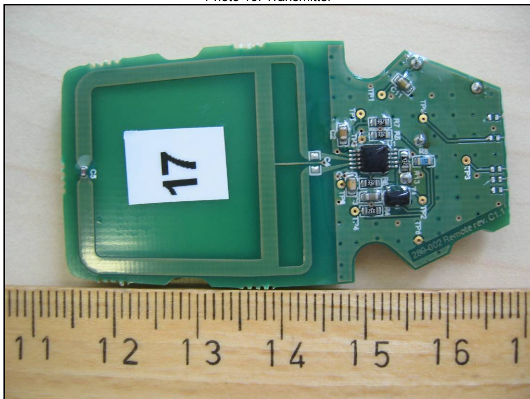
Photo 10: Transmitter
