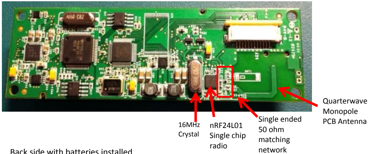
Back side with batteries installed
