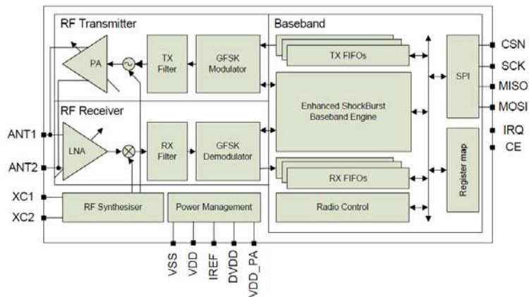
Figure 1. nRF24L01+ block diagram
