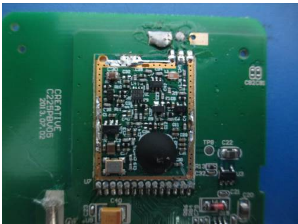
Antenn PCB - Top View
