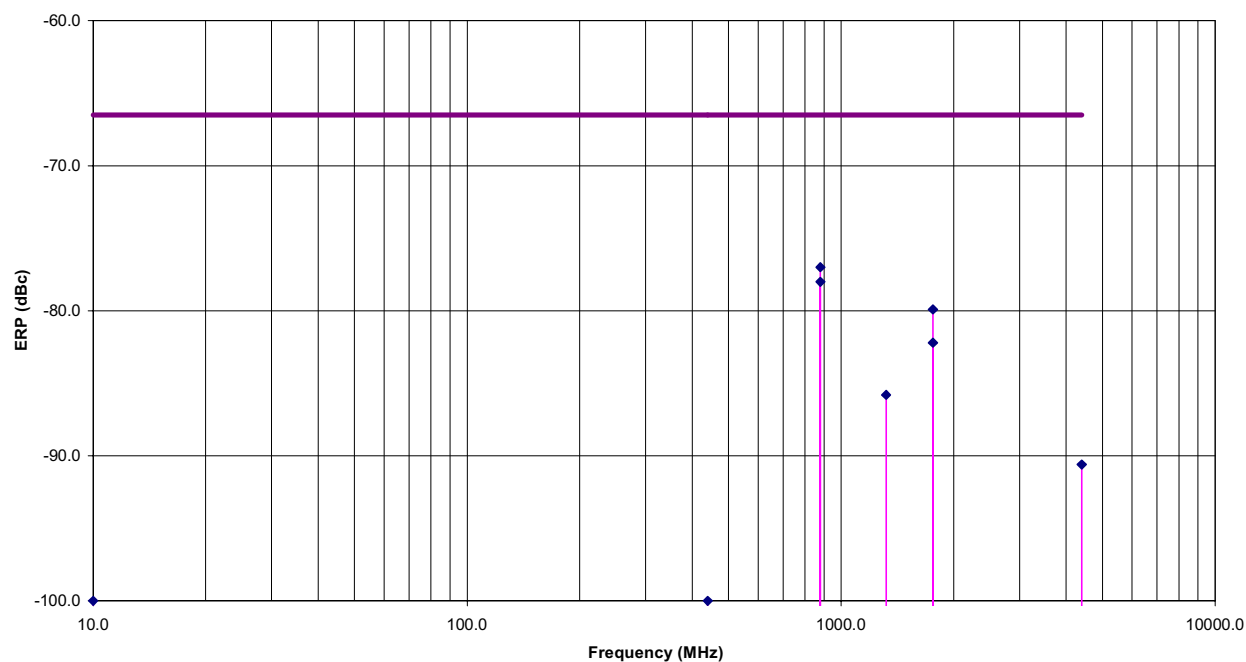
Radiated Emissions Measurements at 3 Meter OFTS ICOM Model IC-F621-2
