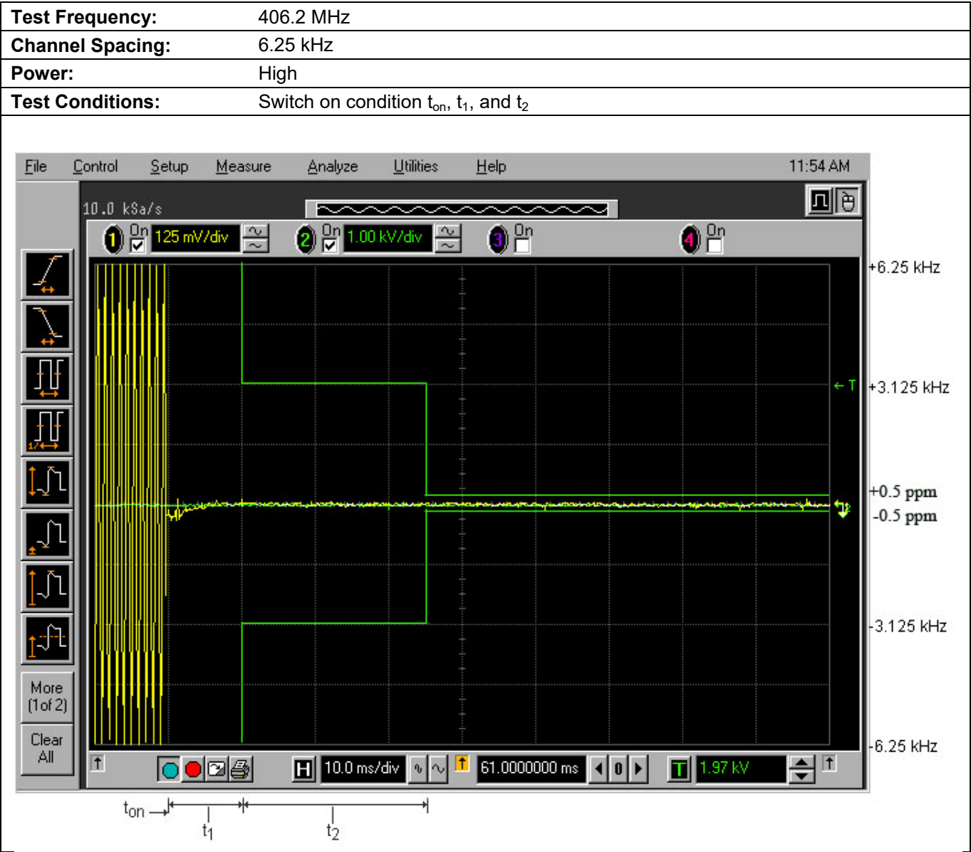
Plot 5.12.3.1. Transient Frequency Behavior for 6.25 kHz Channel Spacing
