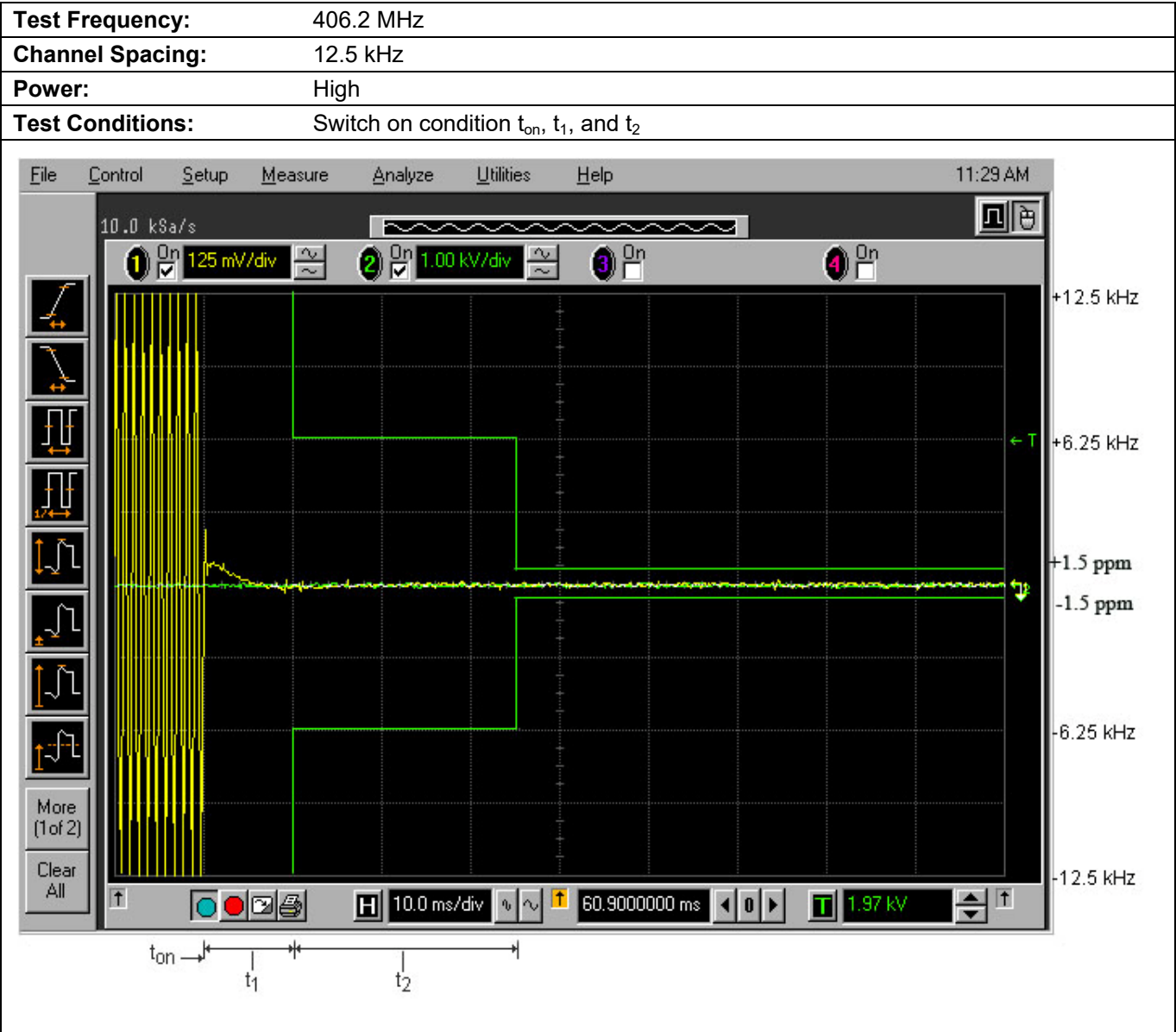
Plot 5.12.3.3. Transient Frequency Behavior for 12.5 kHz Channel Spacing
