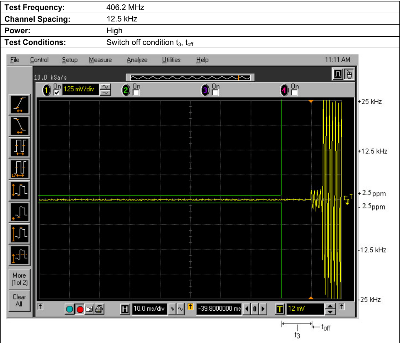
Plot 5.12.3.4. Transient Frequency Behavior for 12.5 kHz Channel Spacing
