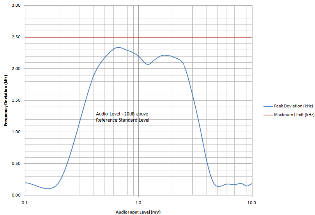
Modulation Limiting IC-6130D NB 12.5kHz
