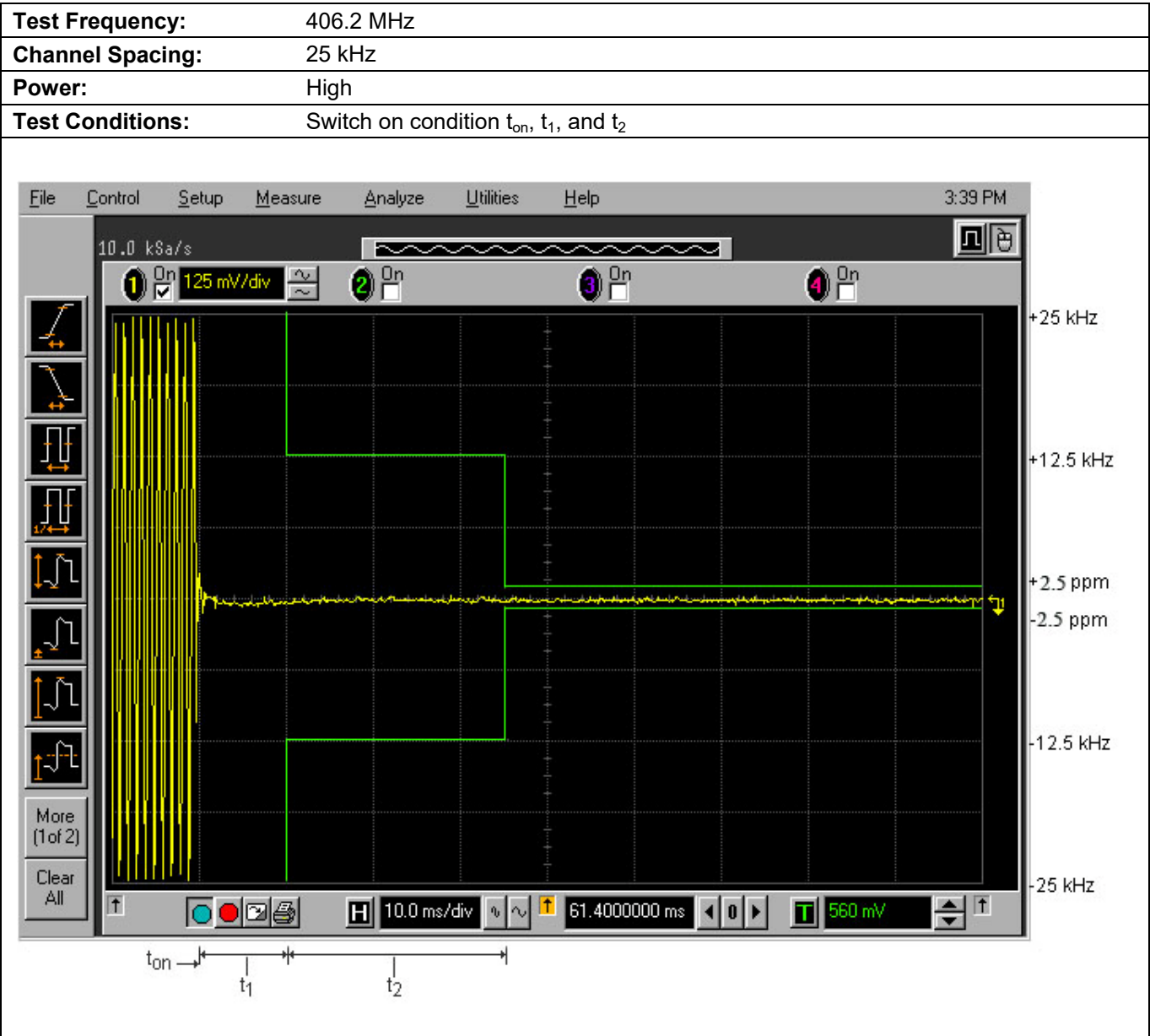
Plot 5.12.3.5. Transient Frequency Behavior for 25 kHz Channel Spacing
