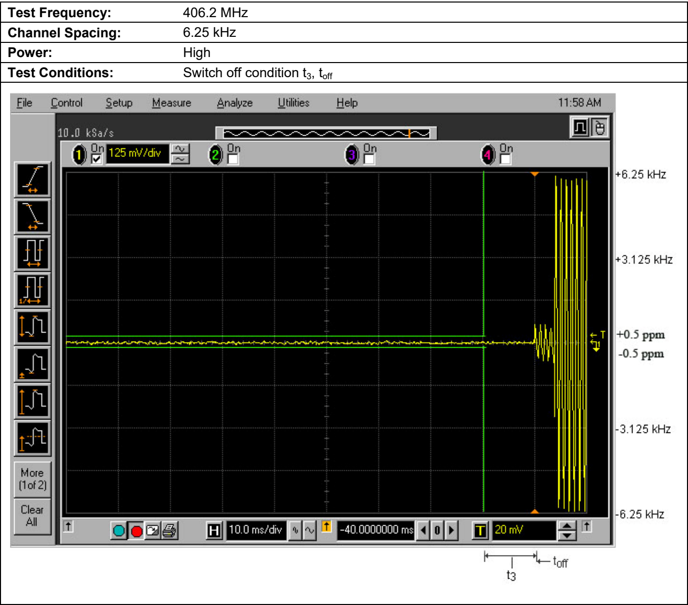
Plot 5.12.3.2. Transient Frequency Behavior for 6.25 kHz Channel Spacing
