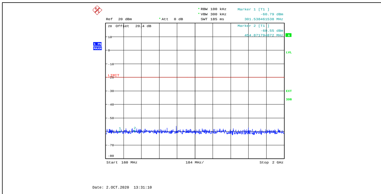
Plot 5.5.4.2. Transmitter Spurious Emissions at Antenna Terminal, Ch 5, 151.820 MHz, High Power 160 MHz – 2 GHz
