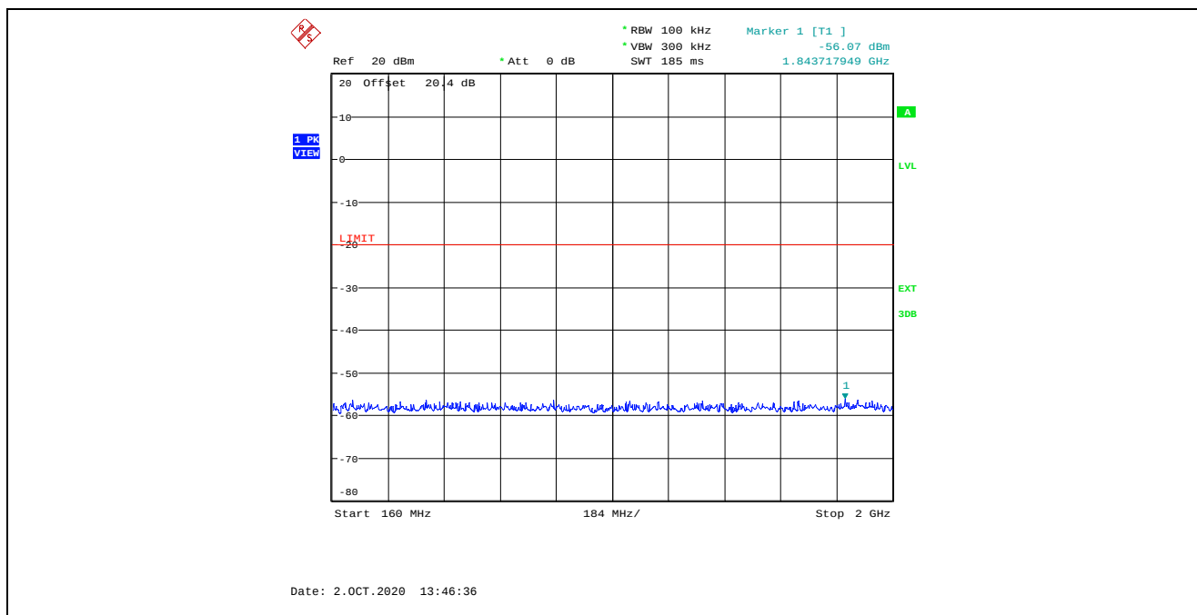
Plot 5.5.4.4. Transmitter Spurious Emissions at Antenna Terminal, Ch 6, 151.820 MHz, Low Power 160 MHz – 2 GHz
