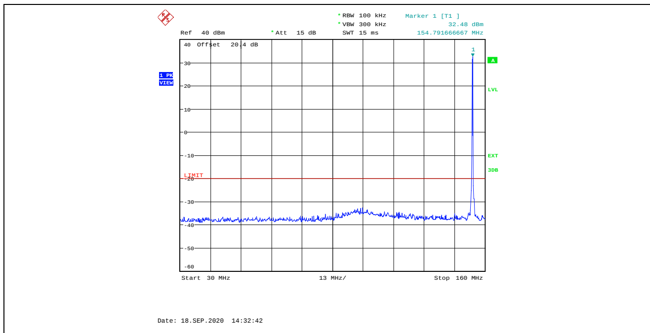
Plot 5.5.4.5. Transmitter Spurious Emissions at Antenna Terminal, Ch 9, 154.600 MHz, High Power 30 – 160 MHz
