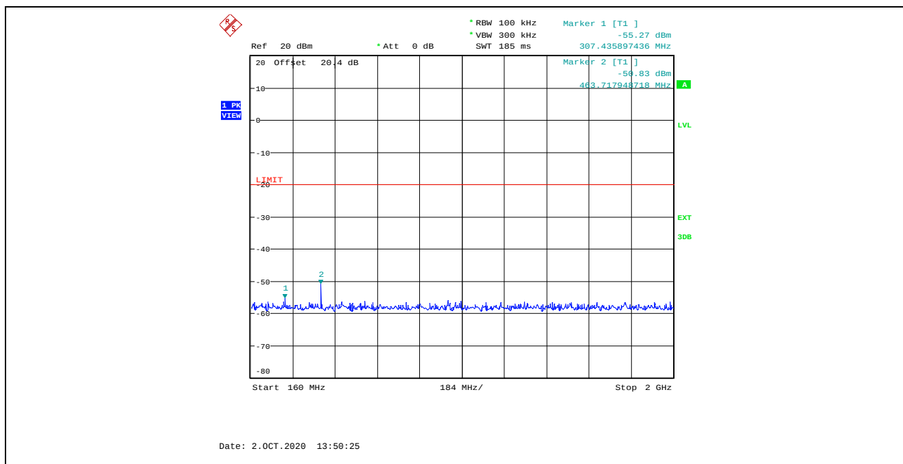
Plot 5.5.4.6. Transmitter Spurious Emissions at Antenna Terminal, Ch 9, 154.600 MHz, High Power 160 MHz – 2 GHz
