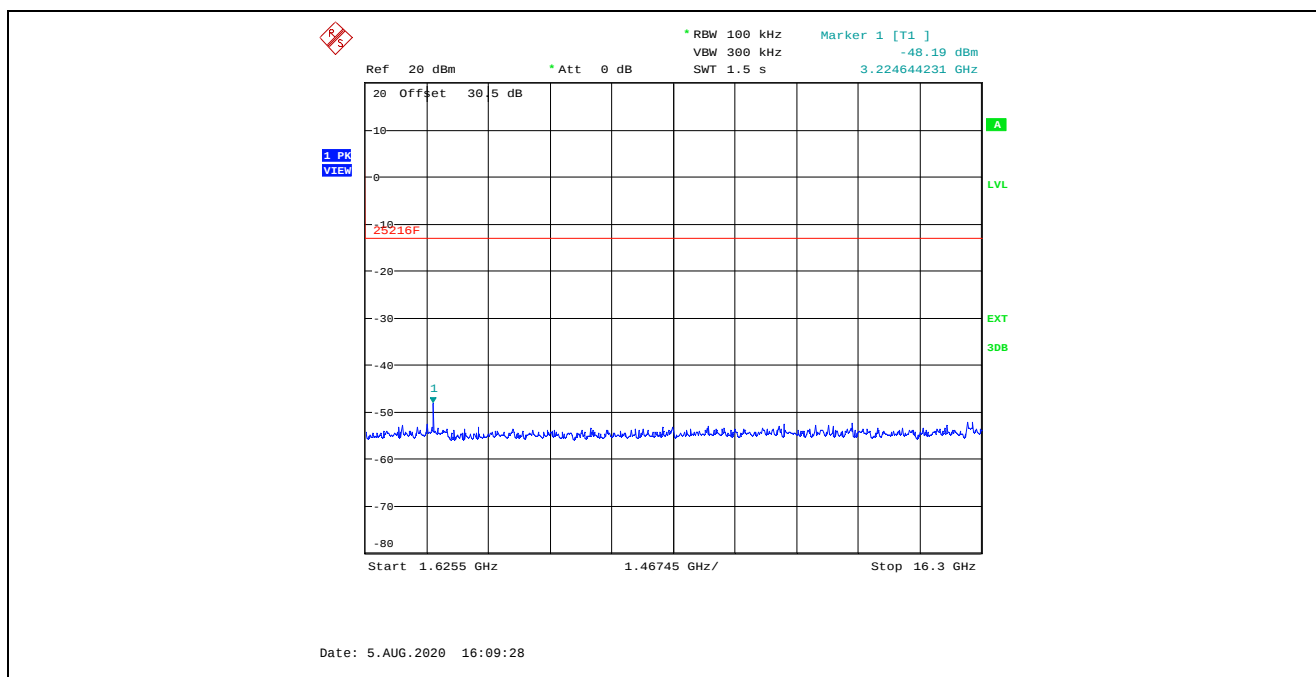
Plot 5.3.4.8. Transmitter Spurious Emissions at Antenna Terminal, Ch 121 1621.020825 MHz 1.6255 GHz – 16.3 GHz
