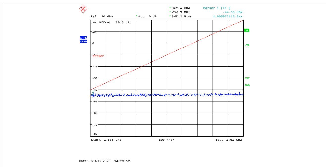
Plot 5.3.4.11. Transmitter Spurious Emissions at Antenna Terminal, Ch 240 1625.979151 MHz 1.605 GHz – 1.61 GHz
