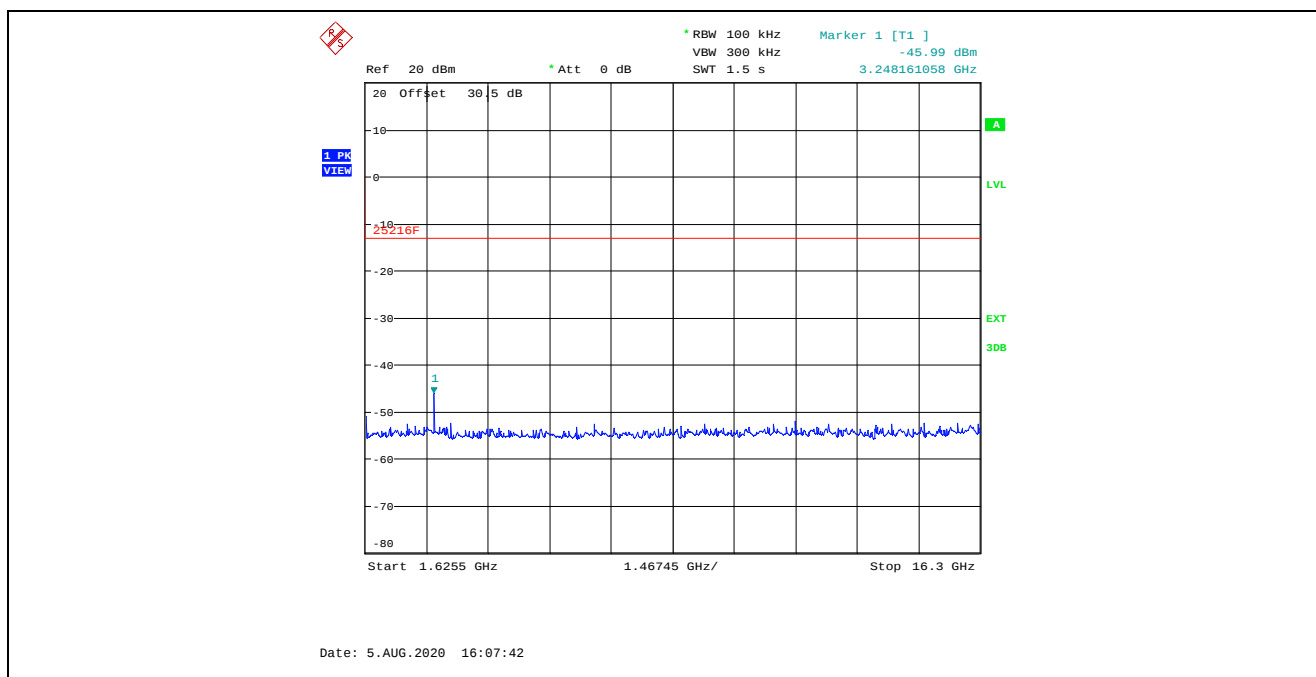
Plot 5.3.4.12. Transmitter Spurious Emissions at Antenna Terminal, Ch 240 1625.979151 MHz 1.6255 GHz – 16.3 GHz
