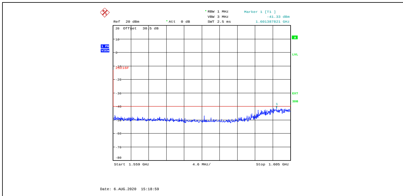
Plot 5.3.4.2. Transmitter Spurious Emissions at Antenna Terminal, Ch 1, 1616.020833 MHz 1.559 GHz – 1.605 GHz
