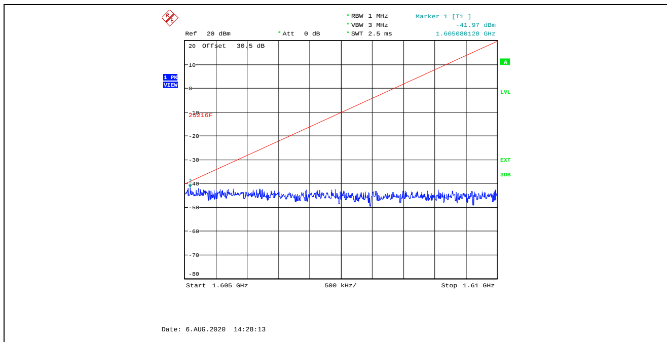
Plot 5.3.4.3. Transmitter Spurious Emissions at Antenna Terminal, Ch 1, 1616.020833 MHz 1.605 GHz – 1.61 GHz
