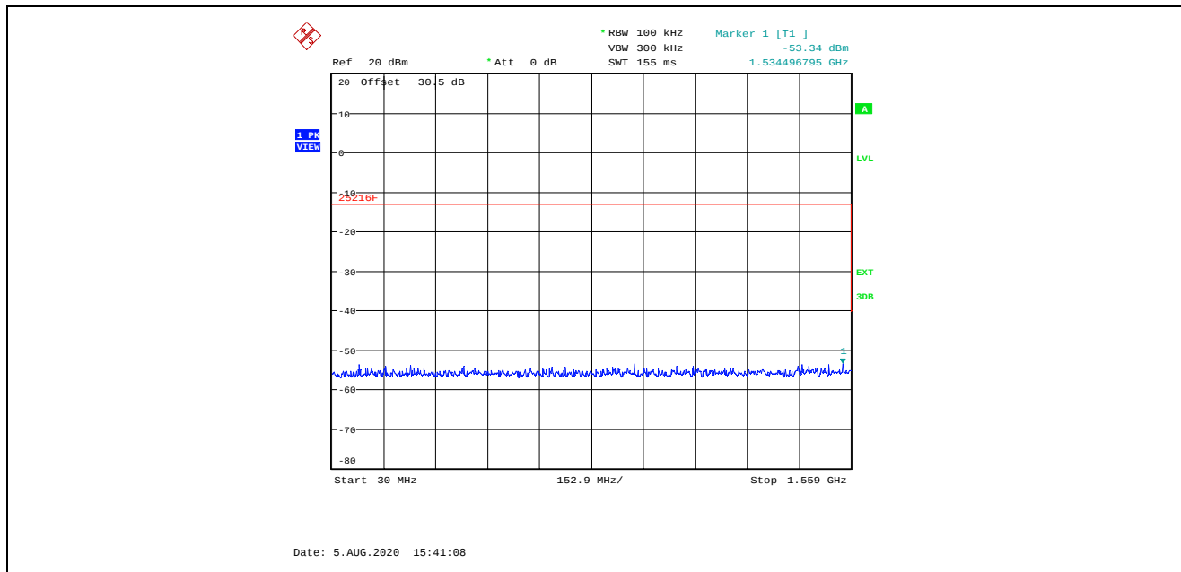
Plot 5.3.4.1. Transmitter Spurious Emissions at Antenna Terminal, Ch 1, 1616.020833 MHz 30 MHz – 1.559 GHz
