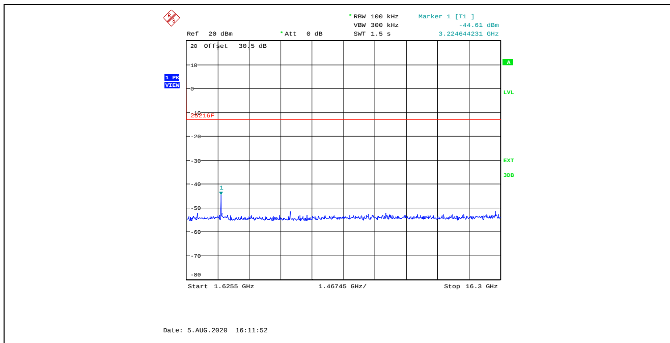
Plot 5.3.4.4. Transmitter Spurious Emissions at Antenna Terminal, Ch 1, 1616.020833 MHz 1.6255 GHz – 16.3 GHz
