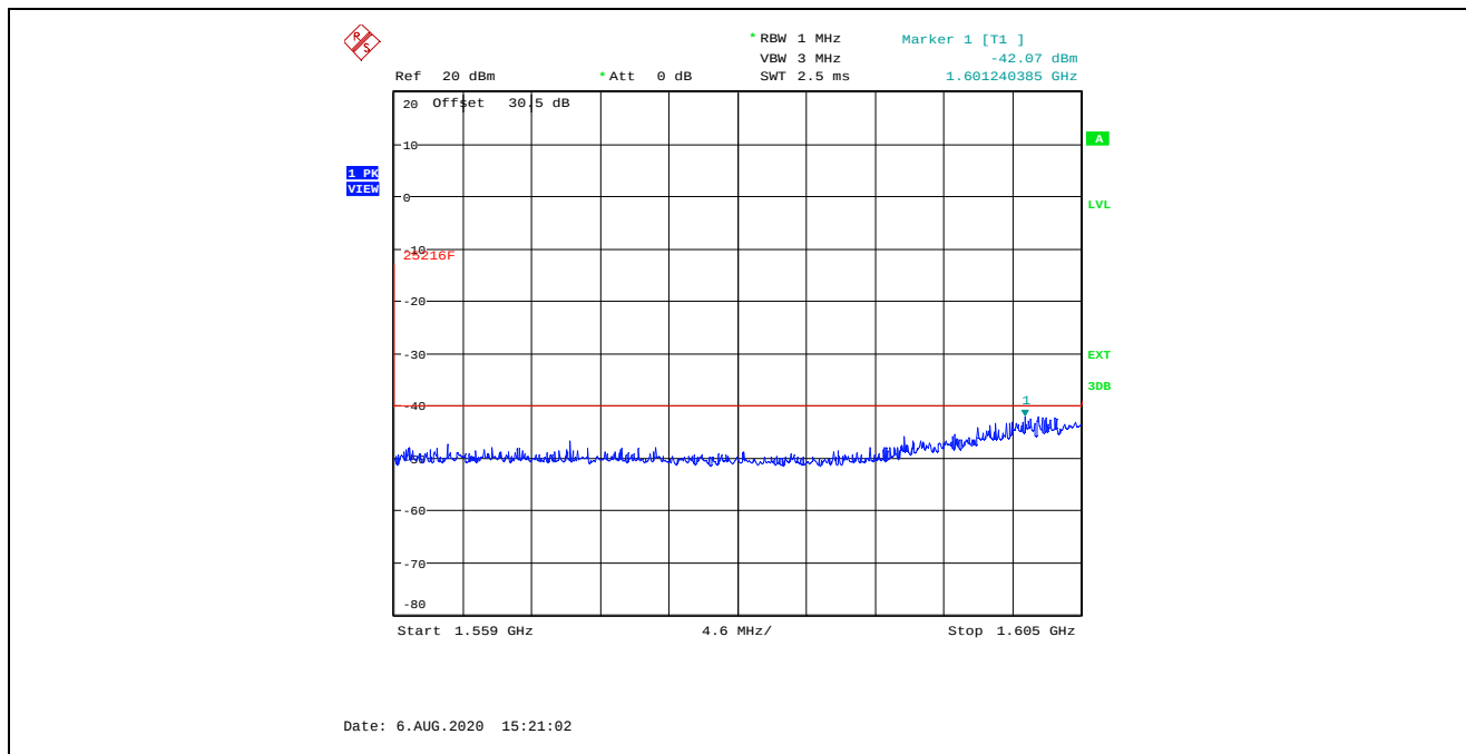
Plot 5.3.4.6. Transmitter Spurious Emissions at Antenna Terminal, Ch 121 1621.020825 MHz 1.559 GHz – 1.605 GHz
