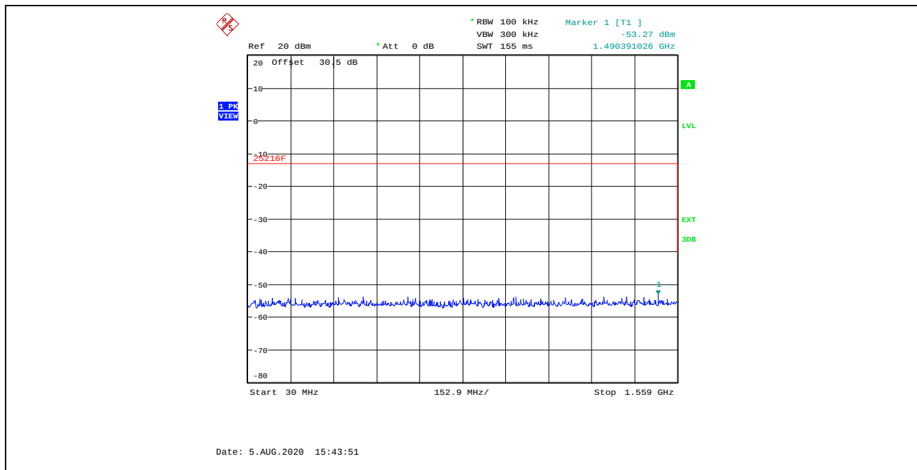
Plot 5.3.4.5. Transmitter Spurious Emissions at Antenna Terminal, Ch 121 1621.020825 MHz 30 MHz – 1.559 GHz
