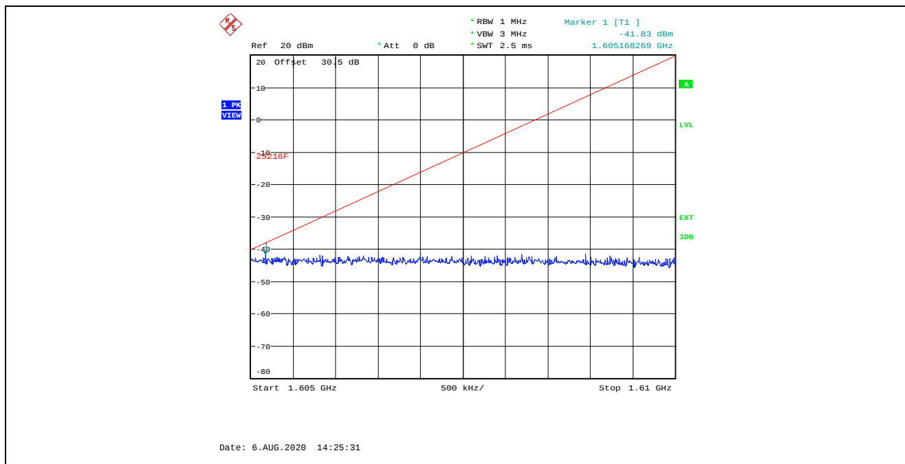
Plot 5.3.4.7. Transmitter Spurious Emissions at Antenna Terminal, Ch 121 1621.020825 MHz 1.605 GHz – 1.61 GHz
