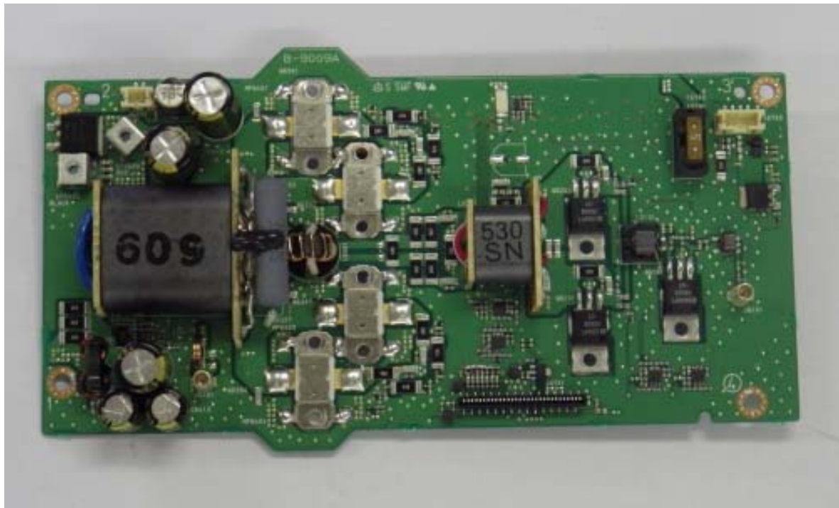
PA unit (top view)
