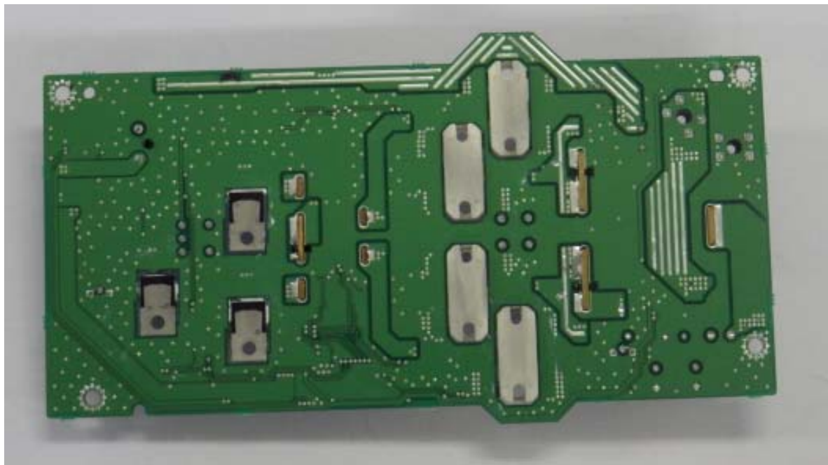
PA unit (bottom view)
