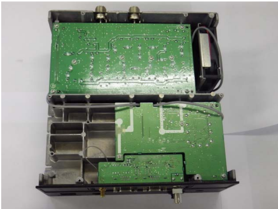
Top View (Inside B)
