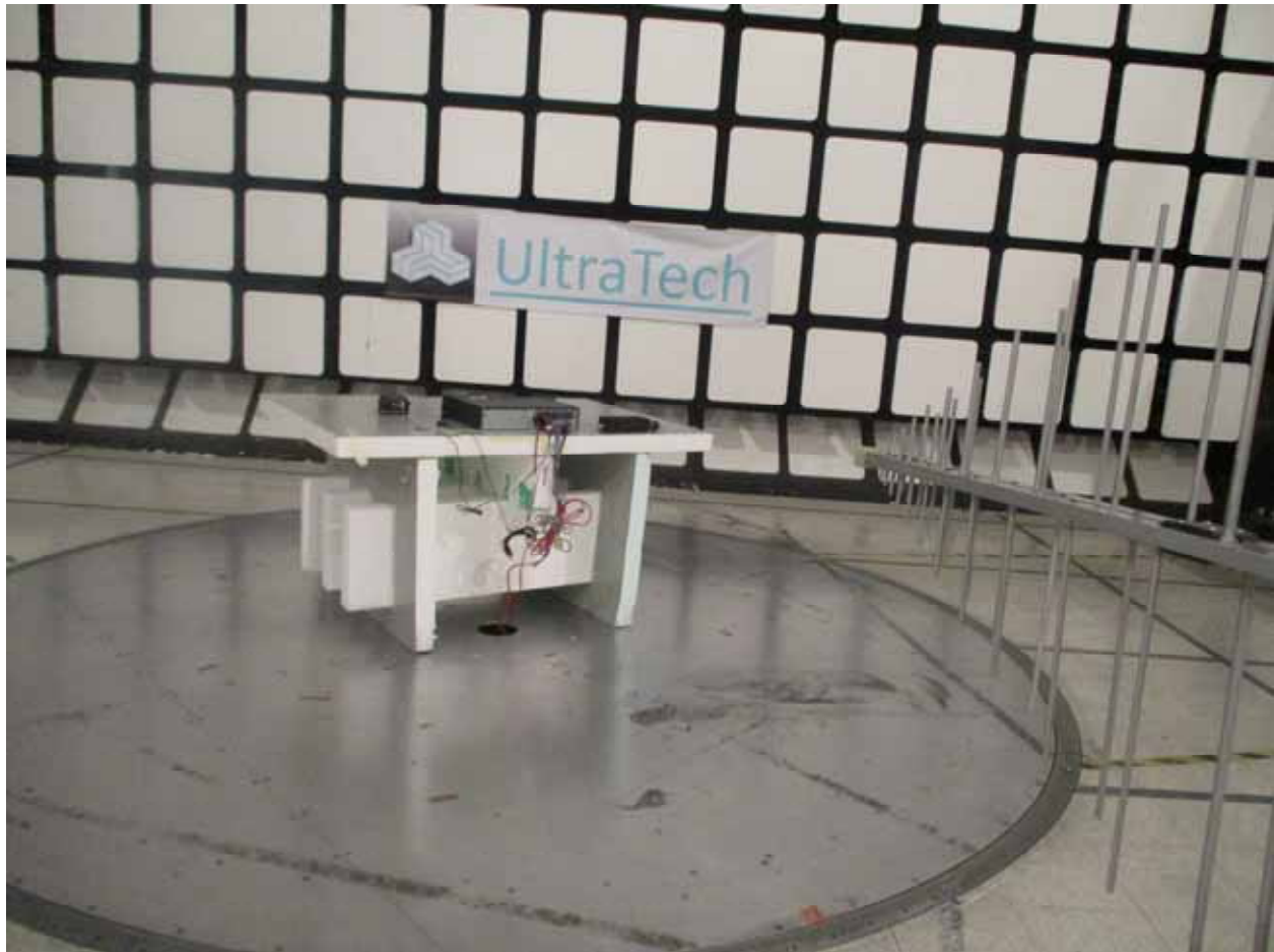
Radiated Setup
