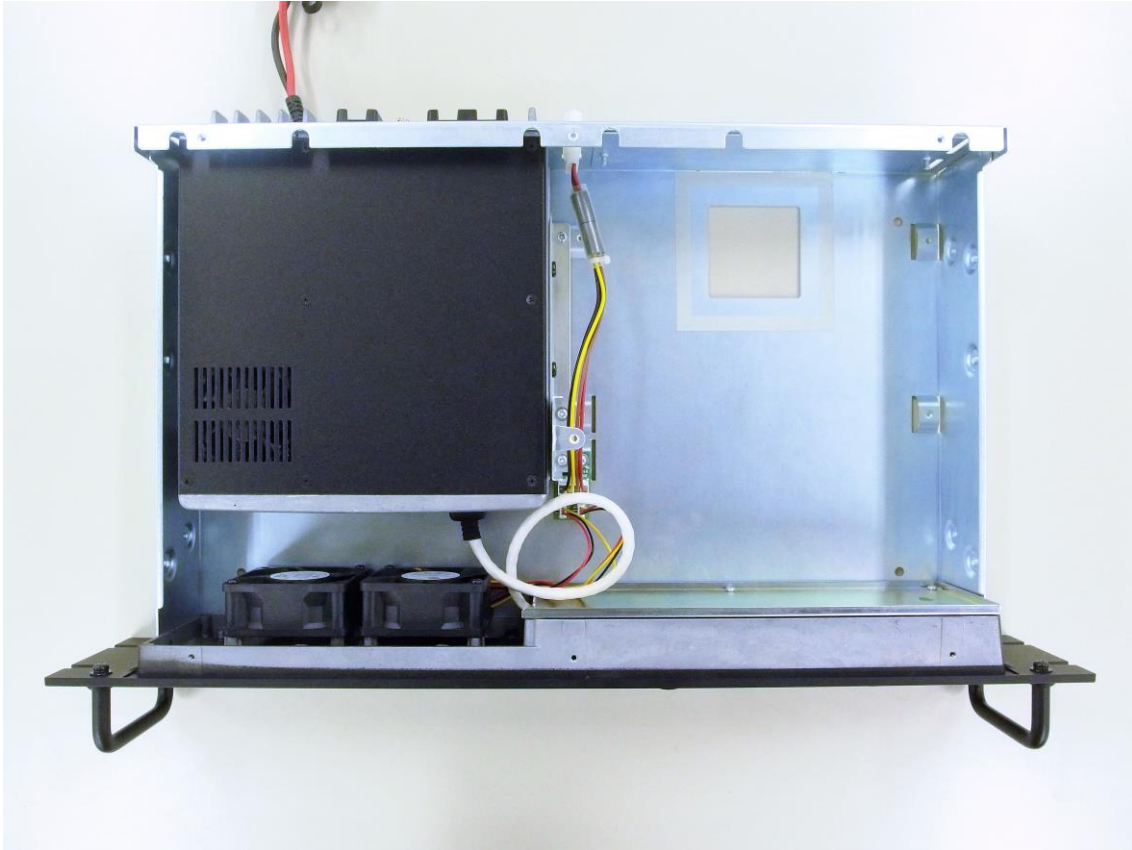
IC-FR6300 COVER OFF
