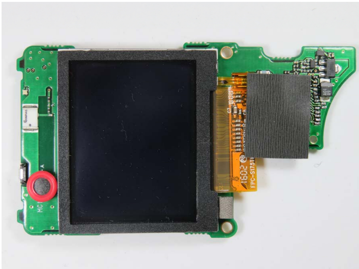
IC-F7040S/T FRONT SIDE A with LCD
