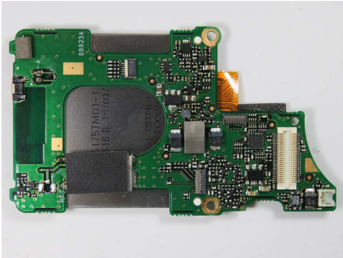
IC-F7040S/T FRONT SIDE B with LCD
