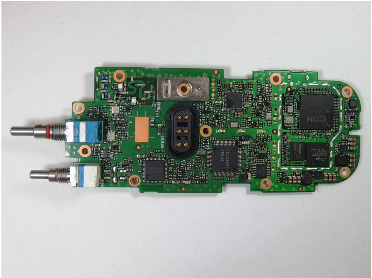
IC-F7040S/T MAIN SIDE B
