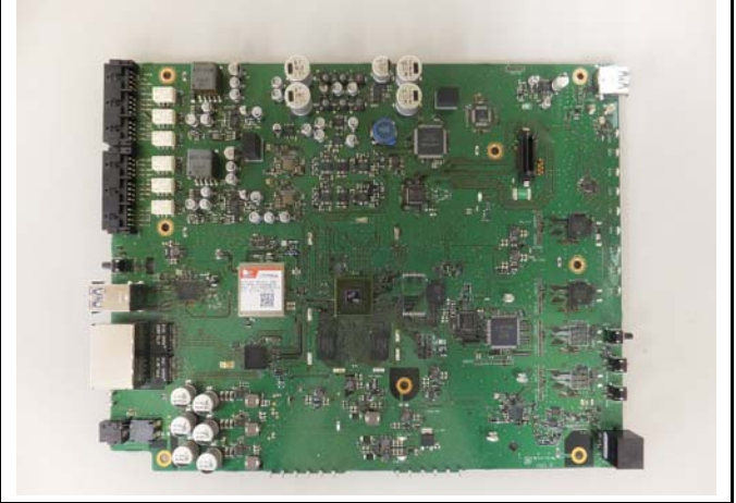
Main Board – Front View
