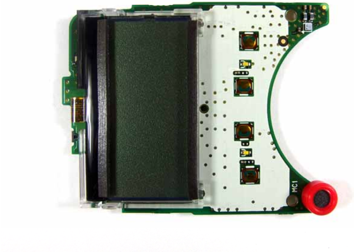
FRONT SIDE A WITH LCD
