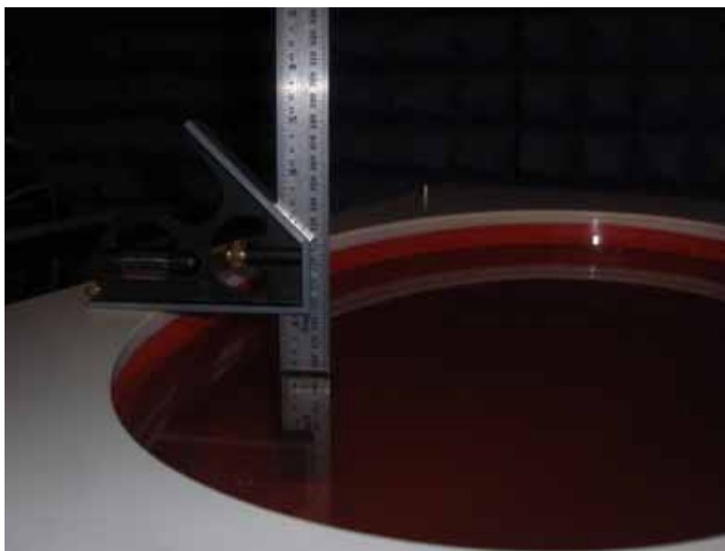
< Phantom filled with Body tissue: liquid level = 150\text{mm} \pm 5\text{mm} >
