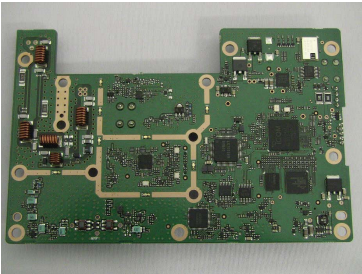
IC-F7510 MAIN UNIT B SIDE
