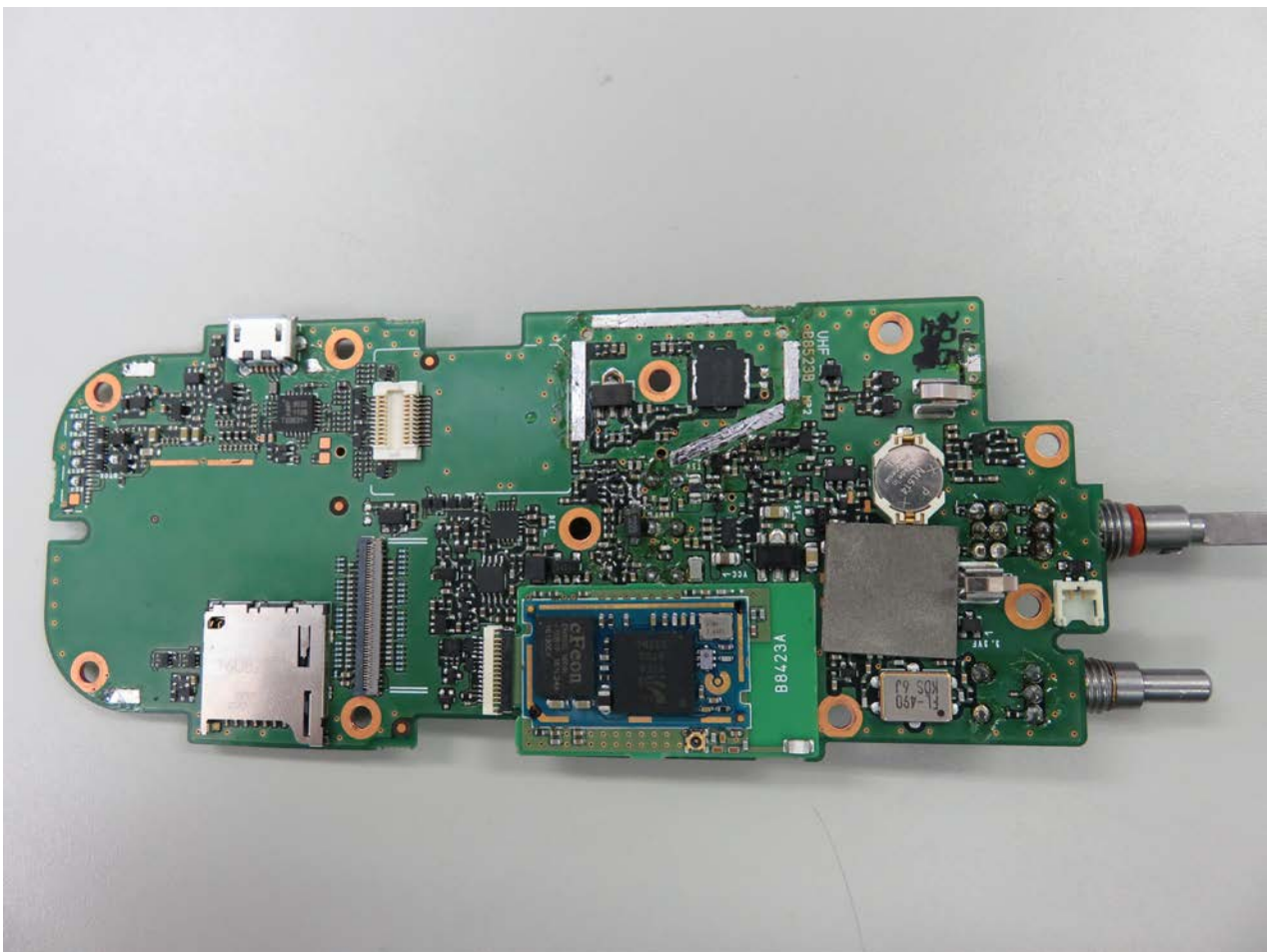
IC-F7020S/T MAIN SIDE A
