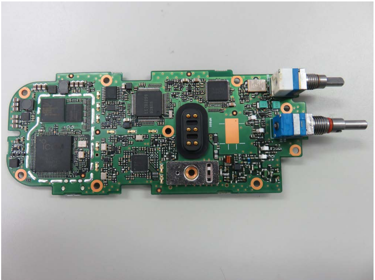
IC-F7020S/T MAIN SIDE B
