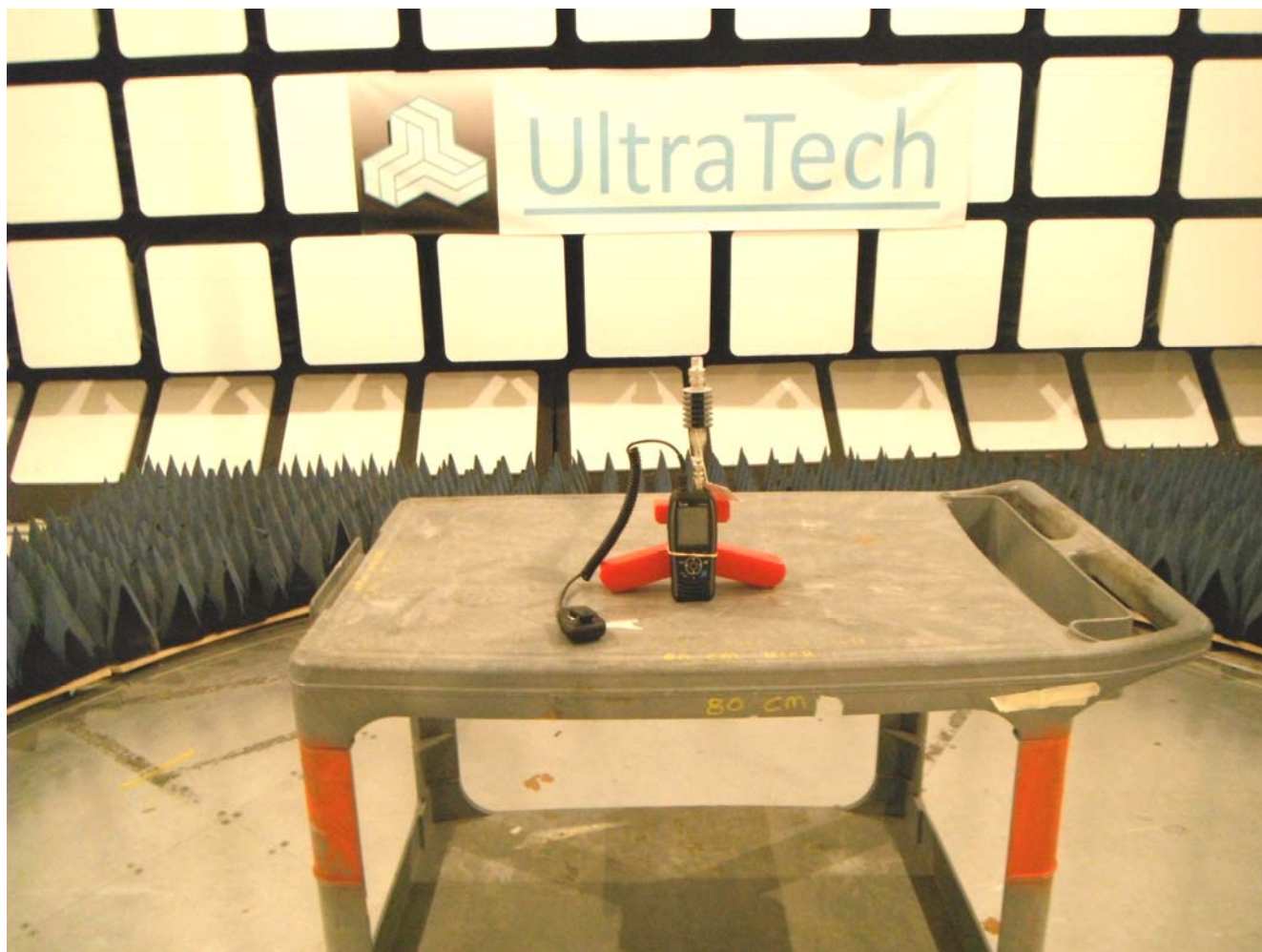
Radiated Emission at 3m (Orthogonal Position 1)
